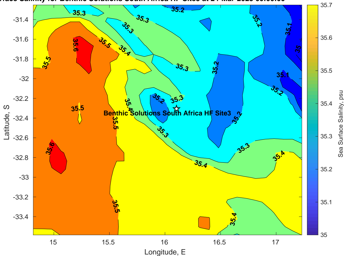
Surface Salinity for Benthic Solutions South Africa HF Site3 at 24-Mar-2025 00:00:00
