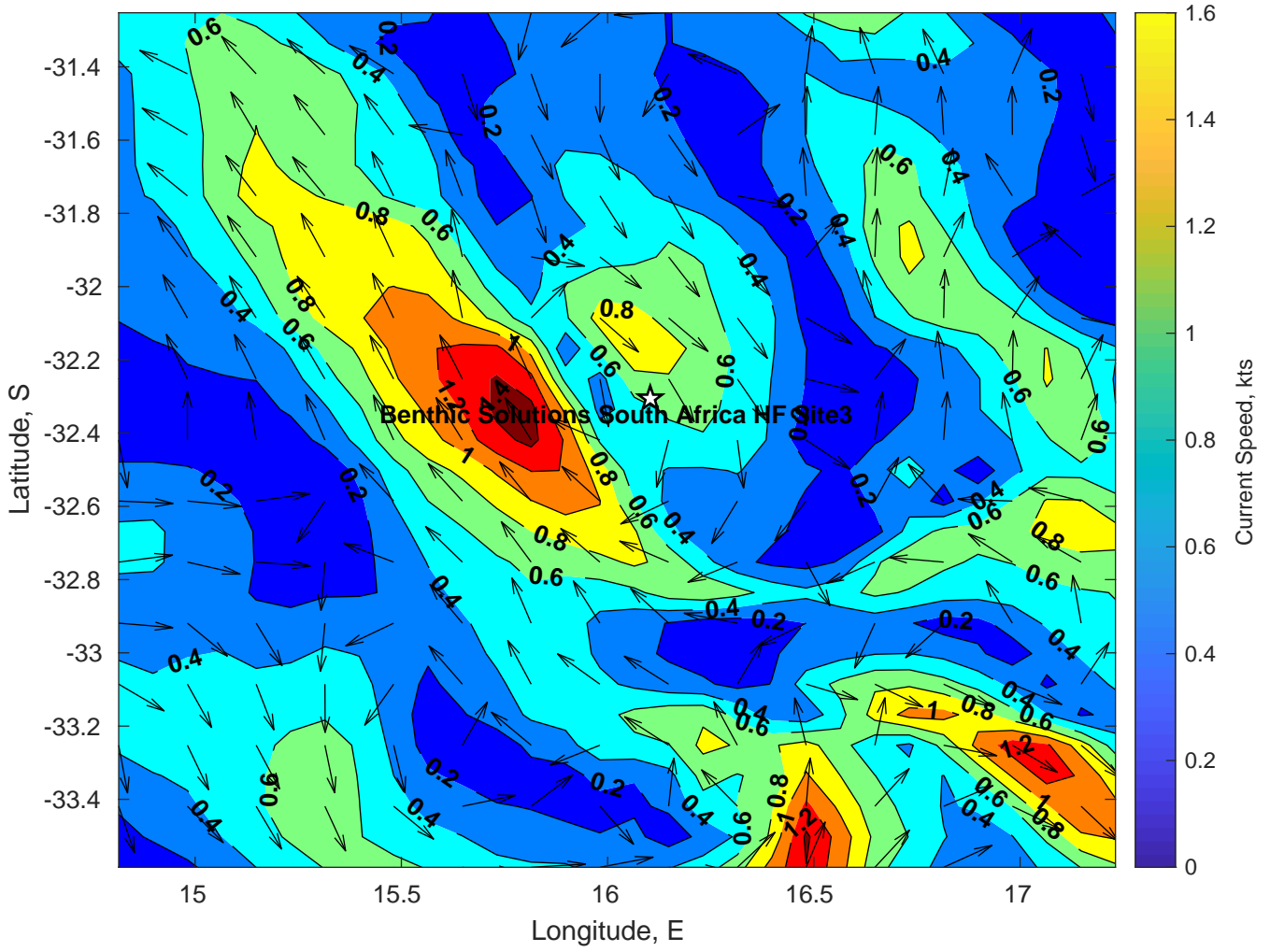
Surface Currents for Benthic Solutions South Africa HF Site3 at 24-Mar-2025 00:00:00
