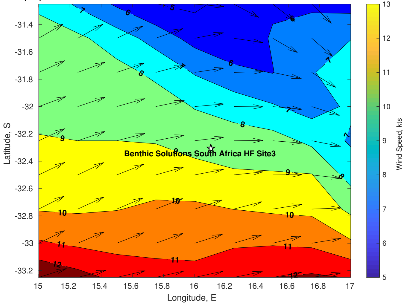
Winds (kts) for Benthic Solutions South Africa HF Site3 at 25-Mar-2025 09:00:00
