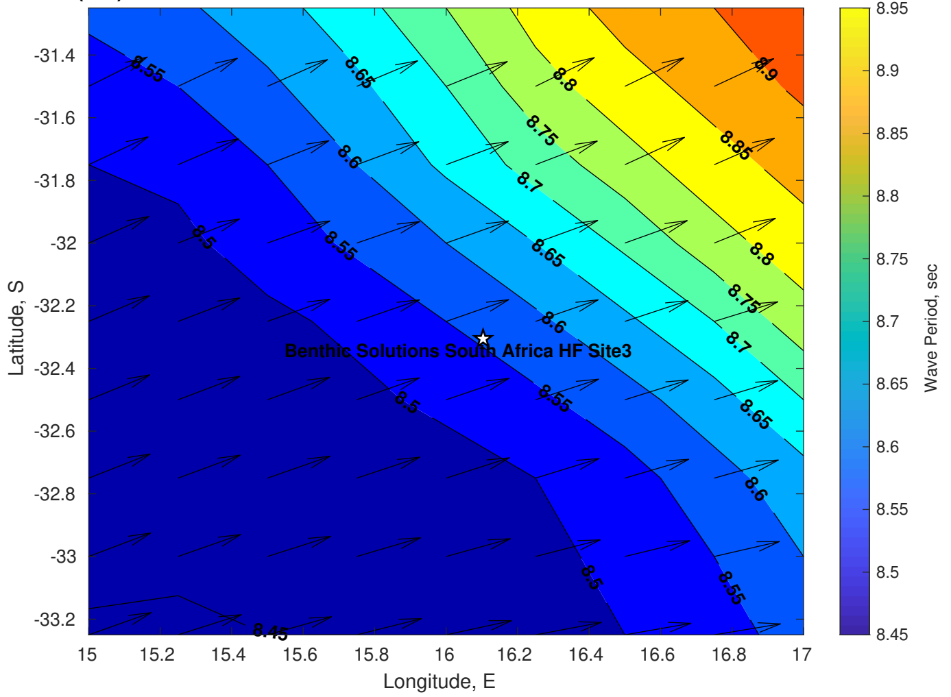
Wave Period (sec) for Benthic Solutions South Africa HF Site3 at 25-Mar-2025 09:00:00
