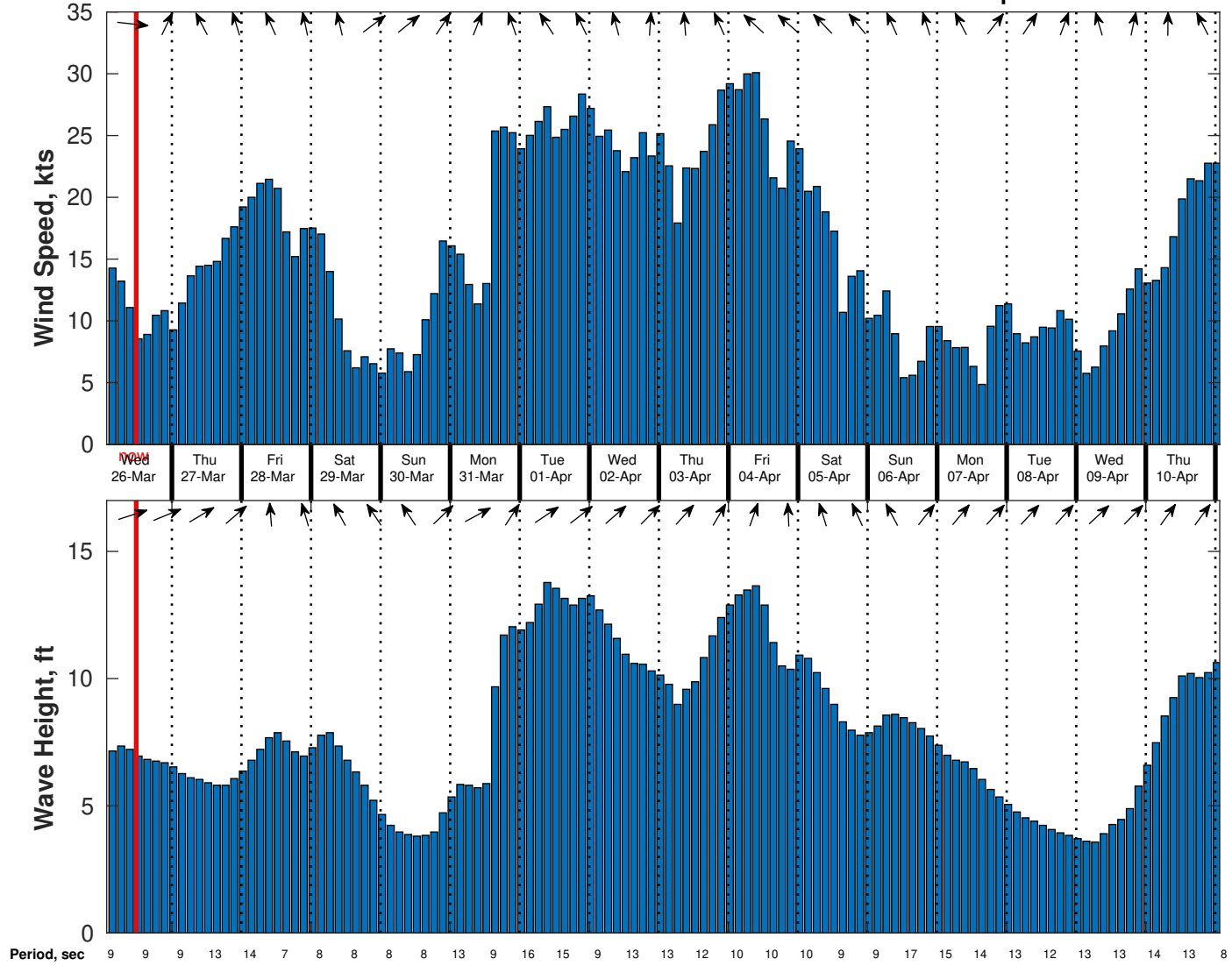
Wind & Wave Forecast for Benthic Solutions South Africa HF Site3 from 25-Mar-2025 02:00:00 to 10-Apr-2025 02:00:00
