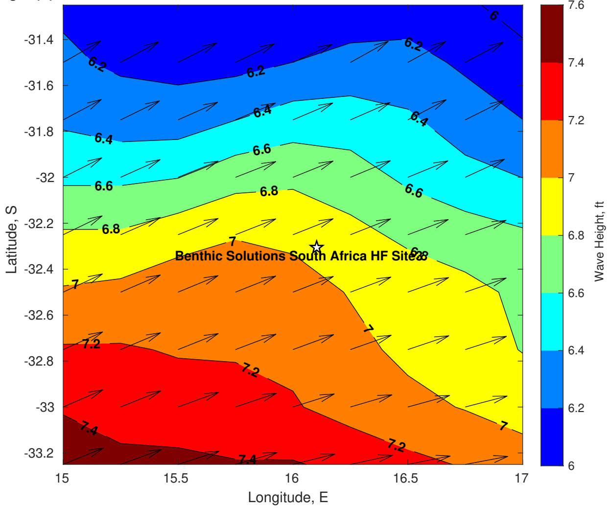
Wave Height (ft) for Benthic Solutions South Africa HF Site3 at 25-Mar-2025 09:00:00
