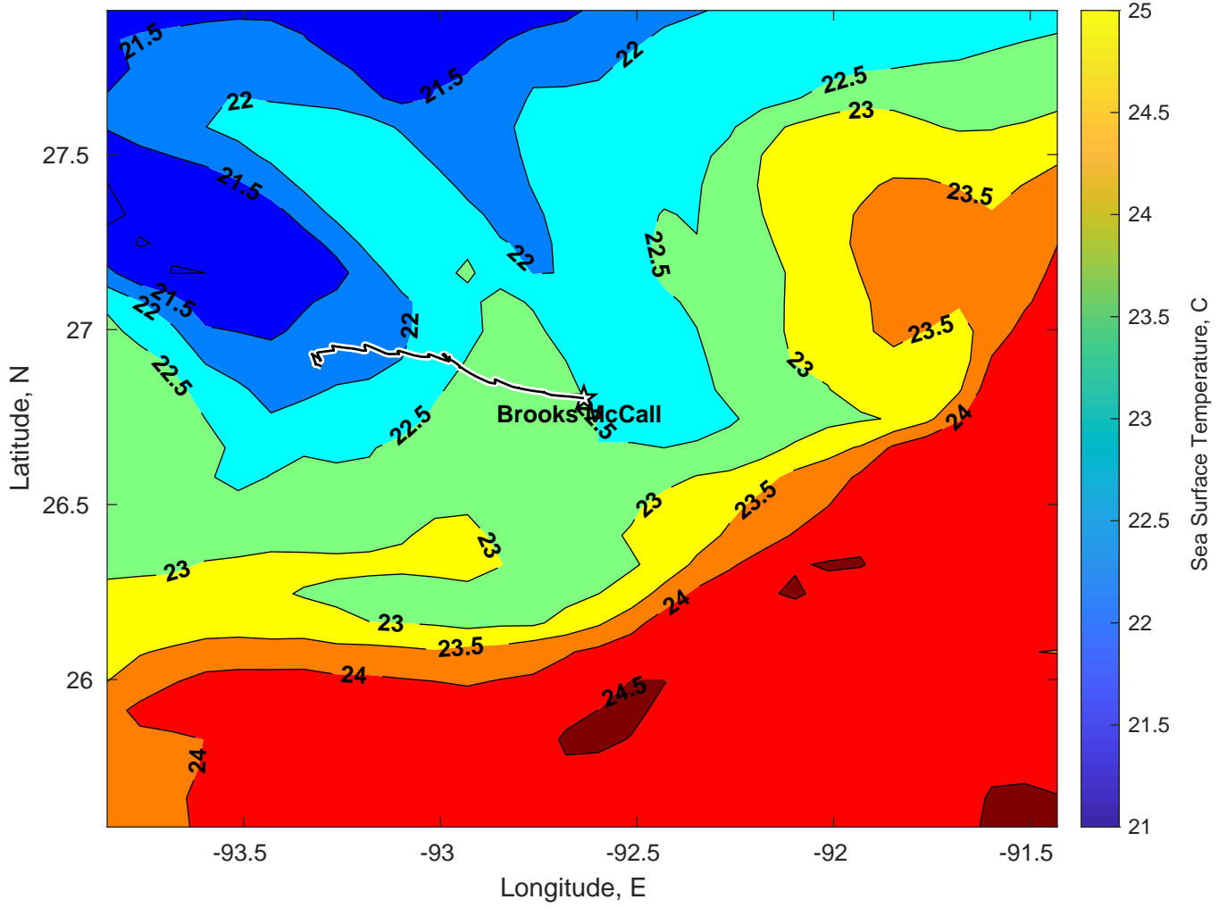
SST for Brooks McCall at 24-Mar-2025 00:00:00
