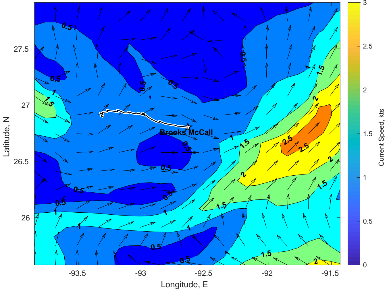
Surface Currents for Brooks McCall at 24-Mar-2025 00:00:00
