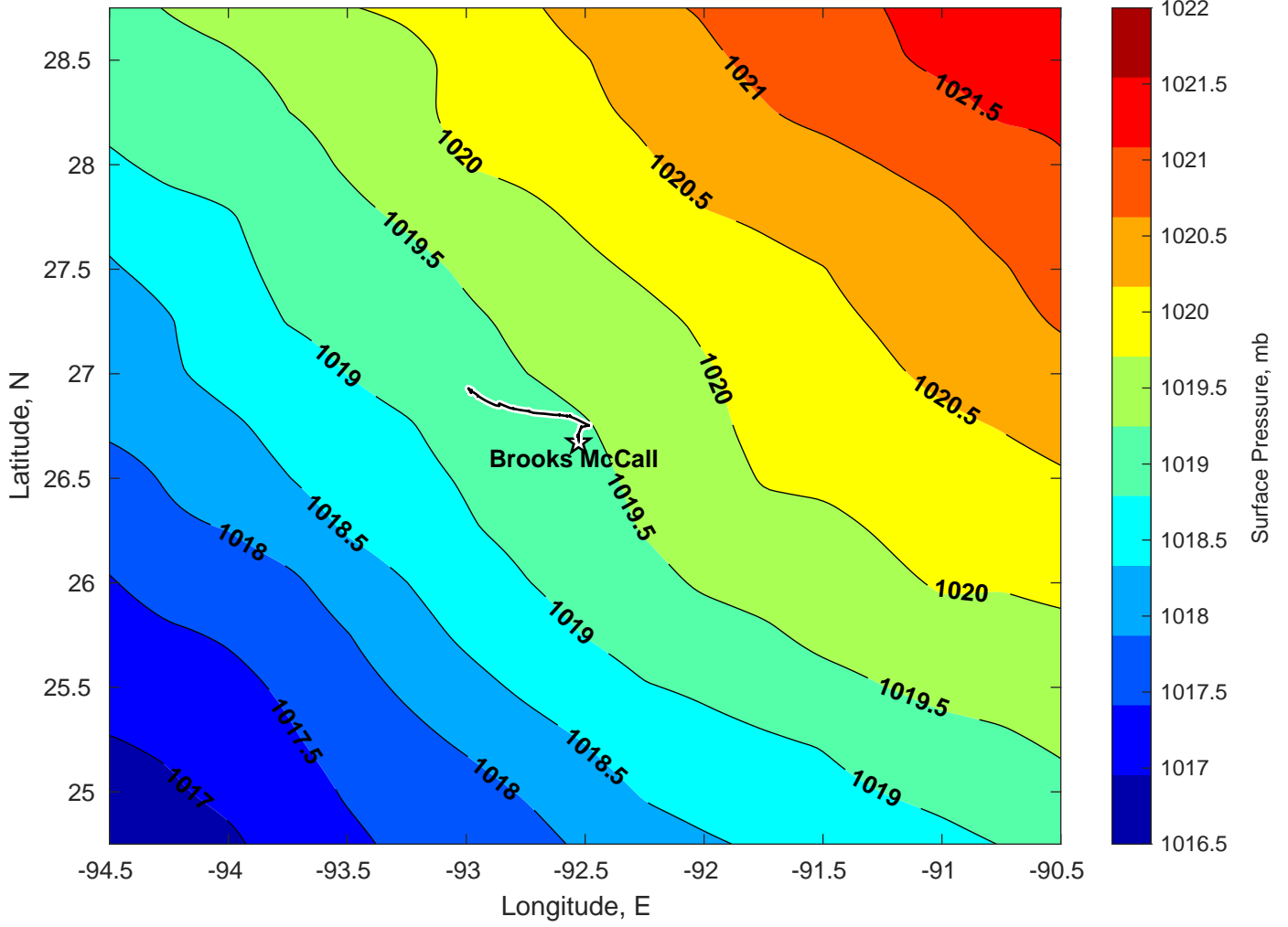
Surface Pressure (mb) for Brooks McCall at 27-Mar-2025 00:00:00
