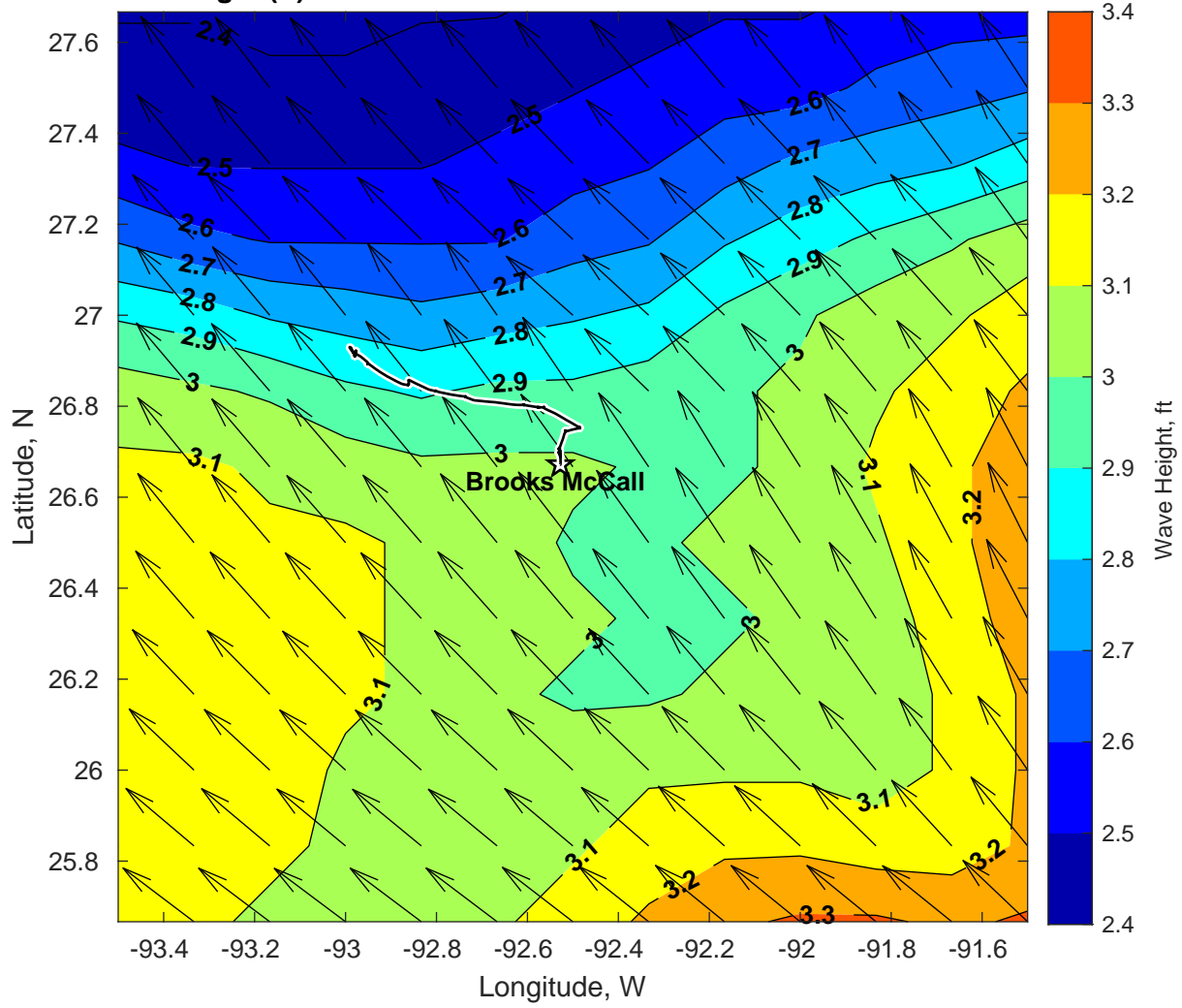
Wave Height (ft) for Brooks McCall at 25-Mar-2025 09:00:00
