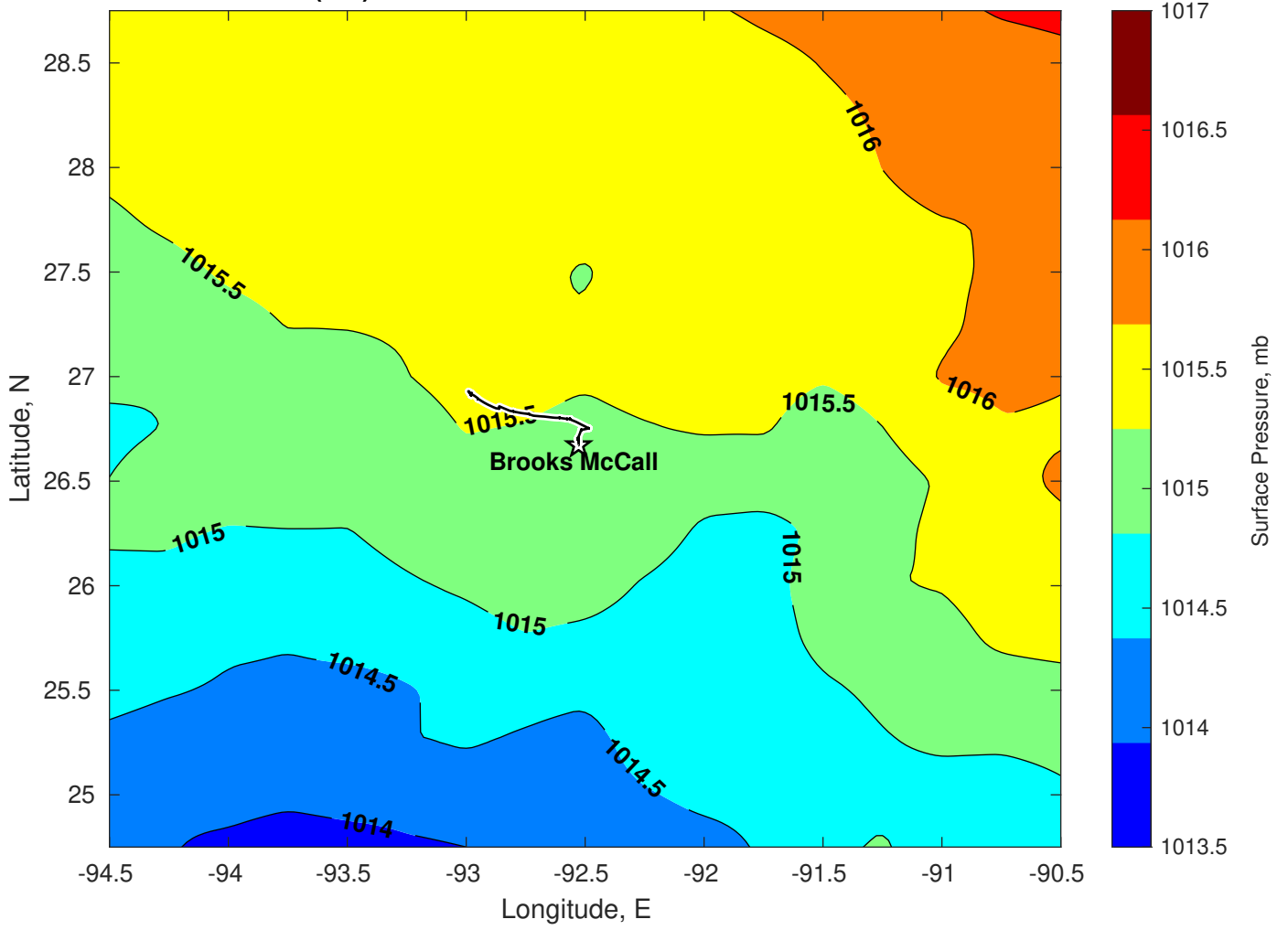
Surface Pressure (mb) for Brooks McCall at 25-Mar-2025 00:00:00
