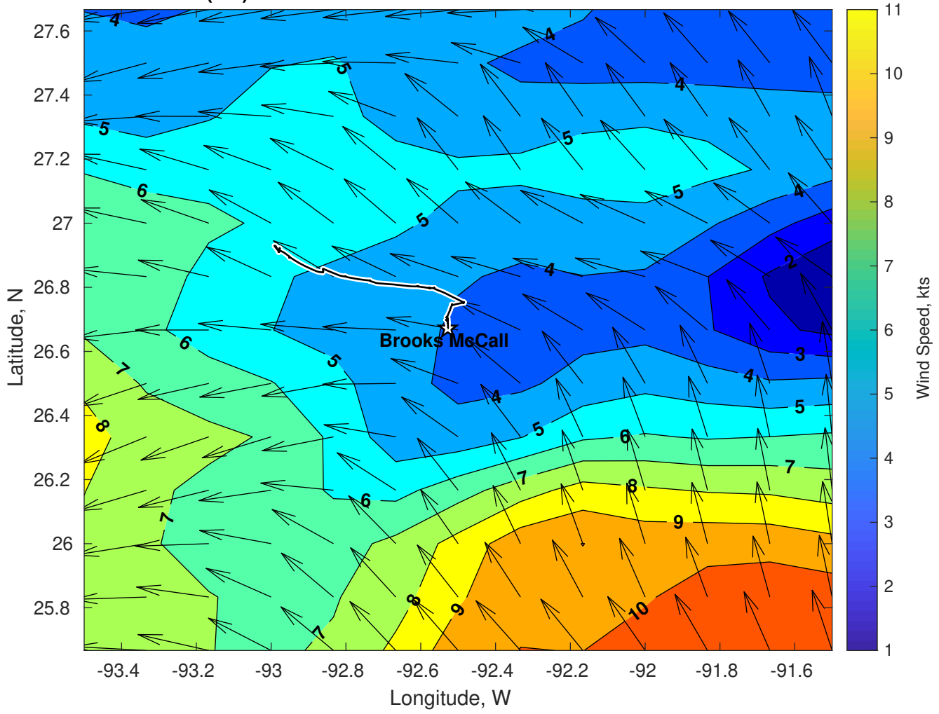
Winds (kts) for Brooks McCall at 25-Mar-2025 09:00:00
