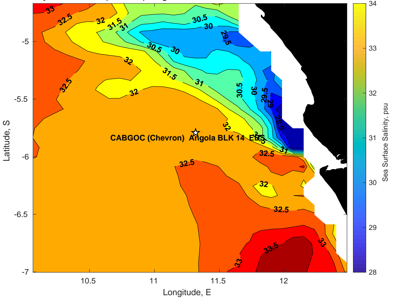
Surface Salinity for CABGOC (Chevron) Angola BLK 14 EBS at 24-Mar-2025 00:00:00
