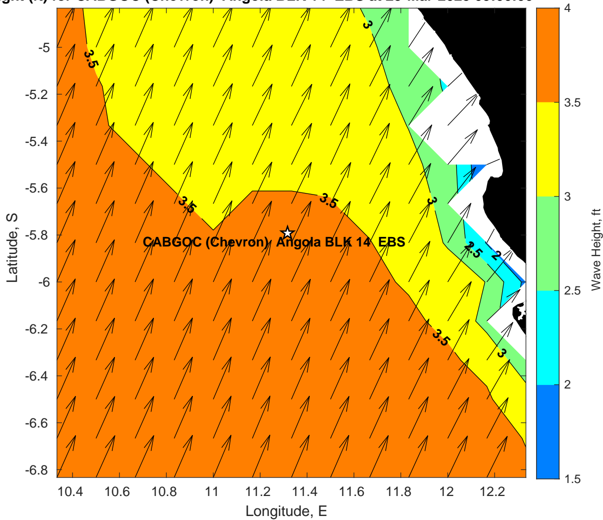
Wave Height (ft) for CABGOC (Chevron) Angola BLK 14 EBS at 25-Mar-2025 09:00:00
