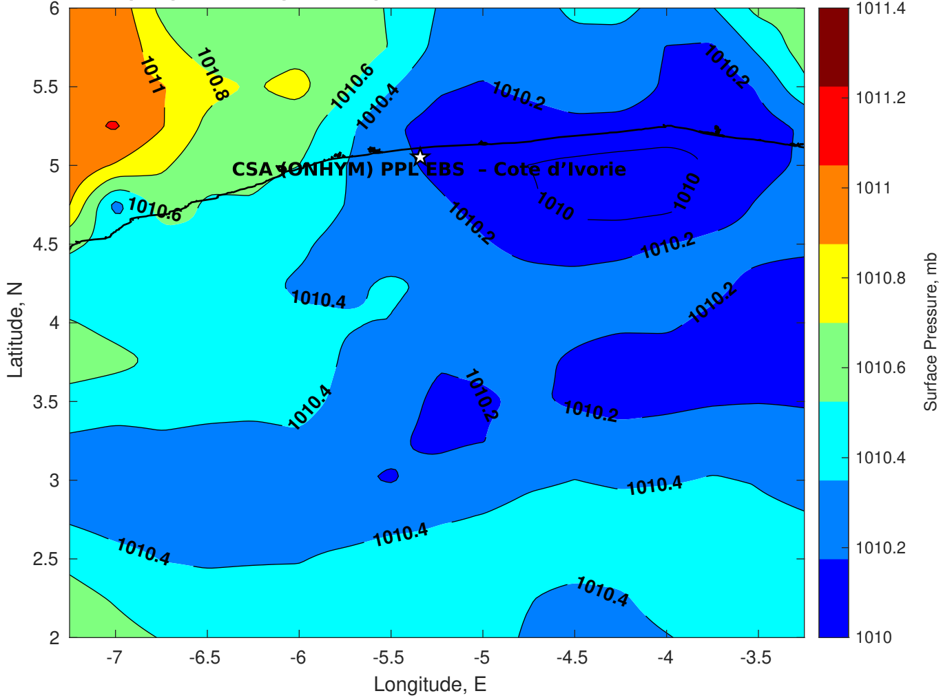
Surface Pressure (mb) for CSA (ONHYM) PPL EBS - Cote d'Ivoire at 27-Mar-2025 00:00:00
