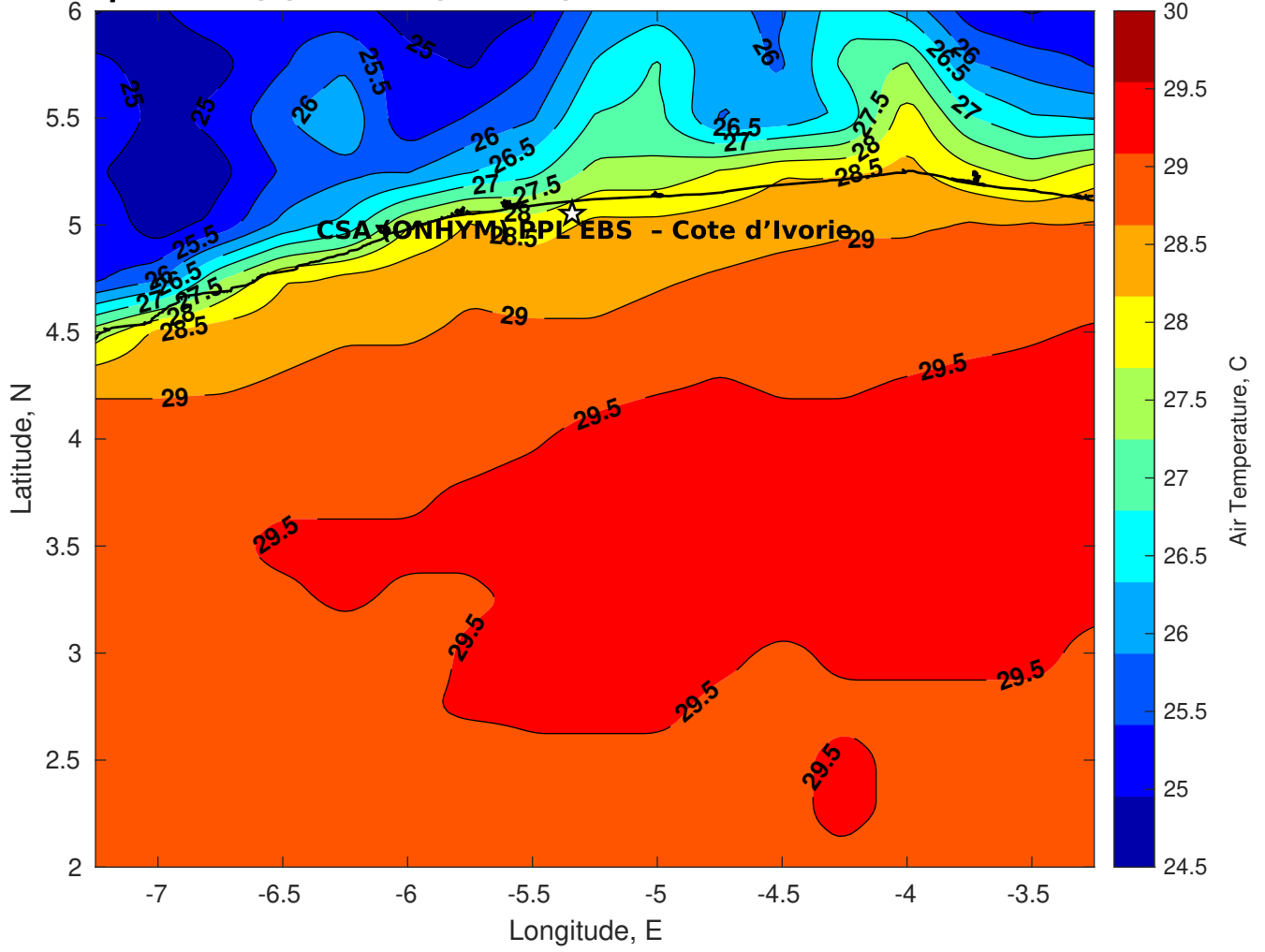
Air Temperature (C) for CSA (ONHYM) PPL EBS - Cote d'Ivoire at 25-Mar-2025
