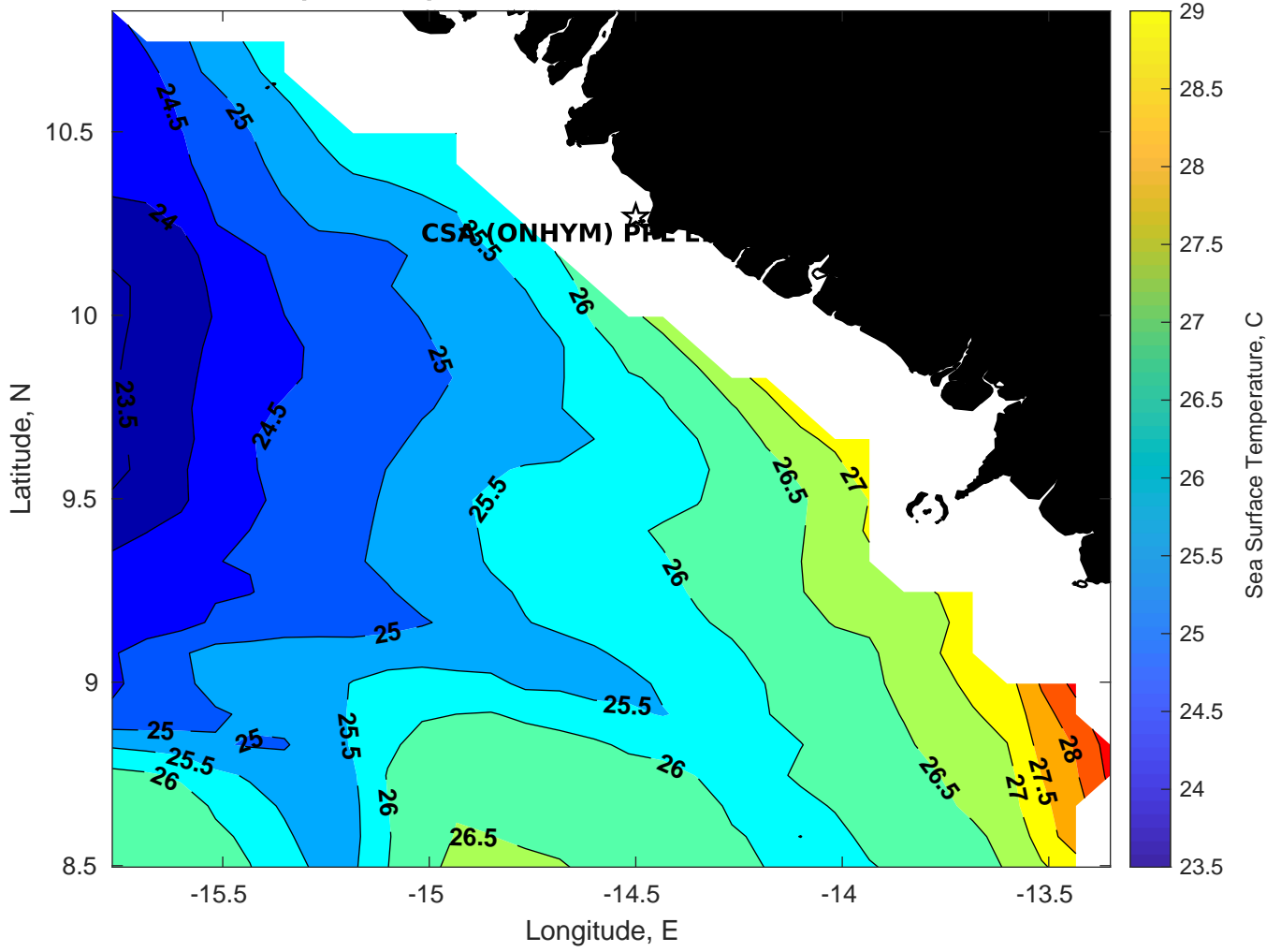
SST for CSA (ONHYM) PPL EBS - Guinea at 24-Mar-2025 00:00:00
