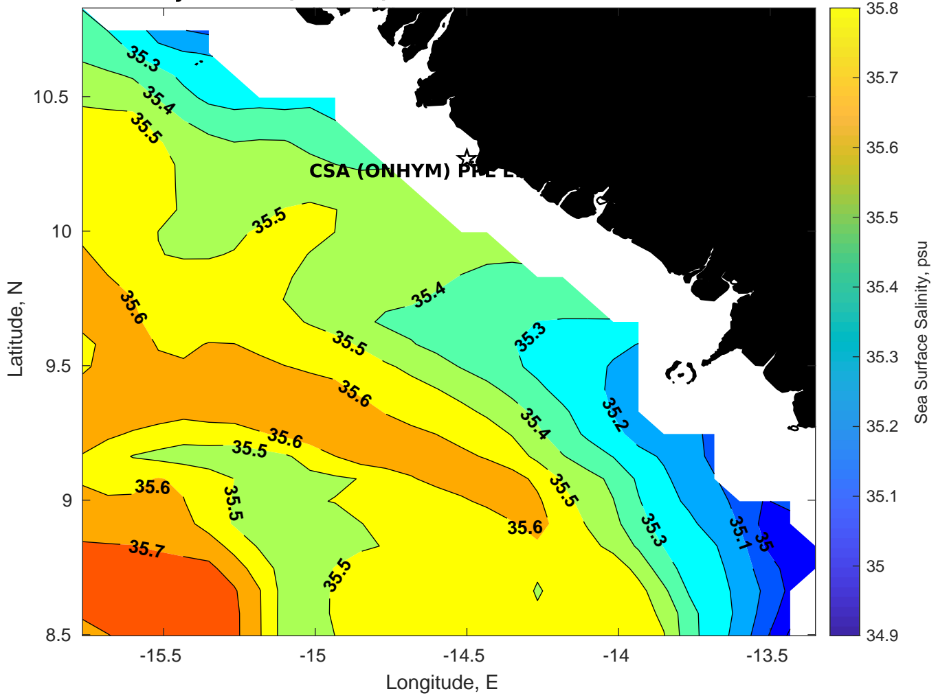
Surface Salinity for CSA (ONHYM) PPL EBS - Guinea at 24-Mar-2025 00:00:00
