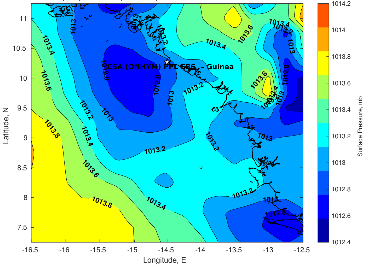
Surface Pressure (mb) for CSA (ONHYM) PPL EBS - Guinea at 26-Mar-2025 00:00:00
