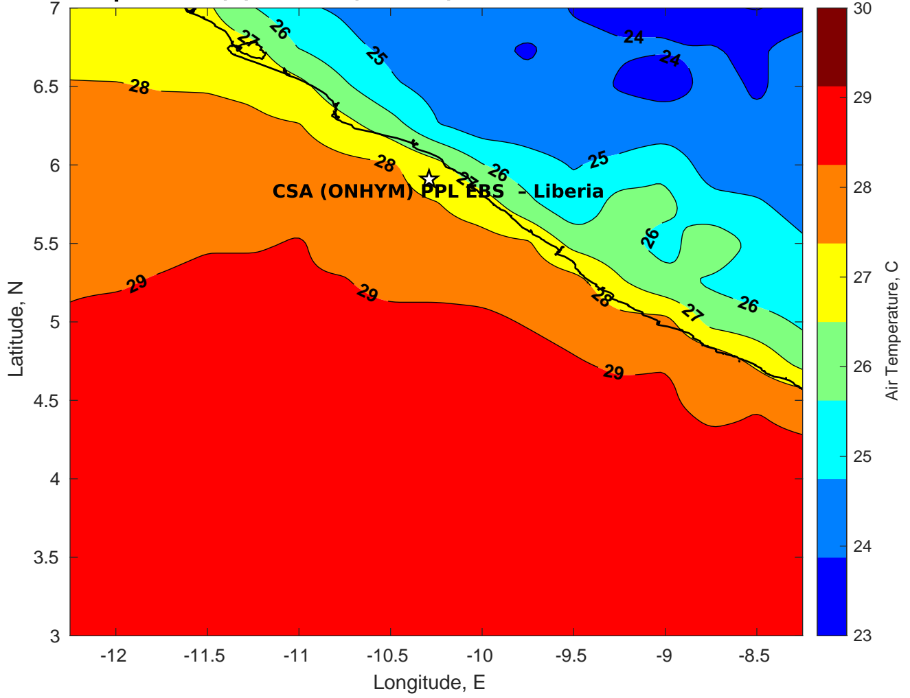
Air Temperature (C) for CSA (ONHYM) PPL EBS - Liberia at 25-Mar-2025
