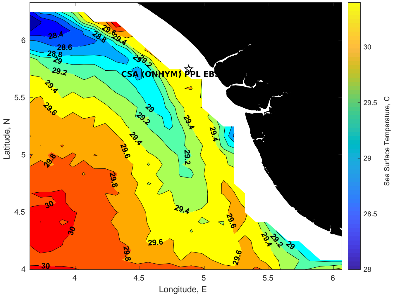
SST for CSA (ONHYM) PPL EBS - Nigeria at 24-Mar-2025 00:00:00
