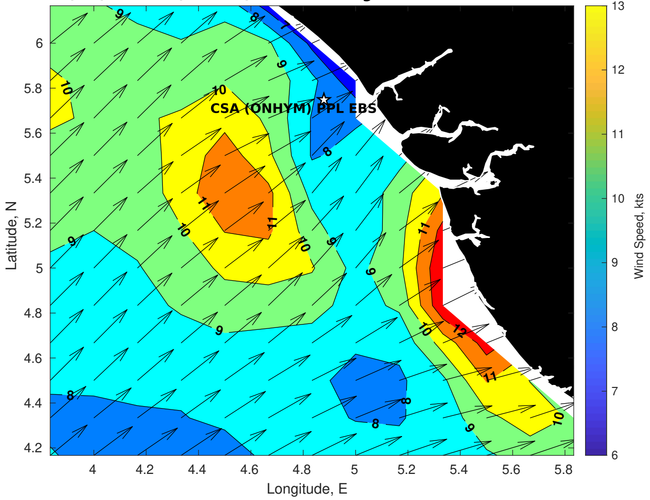
Winds (kts) for CSA (ONHYM) PPL EBS - Nigeria at 25-Mar-2025 09:00:00
