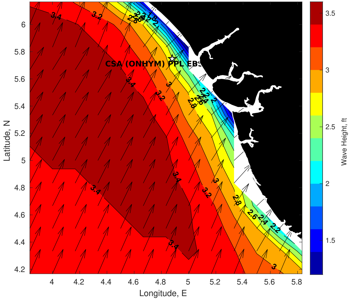
Wave Height (ft) for CSA (ONHYM) PPL EBS - Nigeria at 25-Mar-2025 09:00:00
