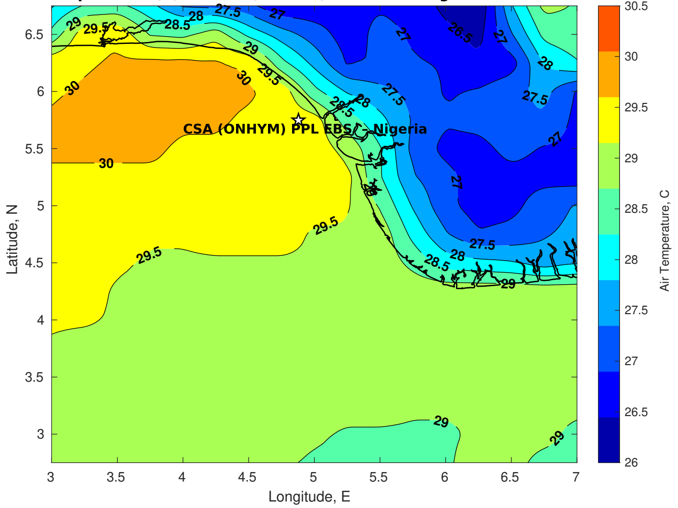
Air Temperature (C) for CSA (ONHYM) PPL EBS - Nigeria at 25-Mar-2025
