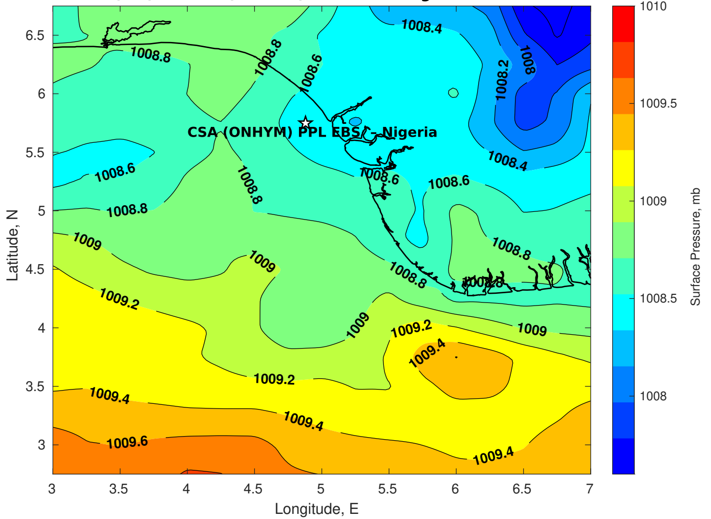
Surface Pressure (mb) for CSA (ONHYM) PPL EBS - Nigeria at 27-Mar-2025 00:00:00
