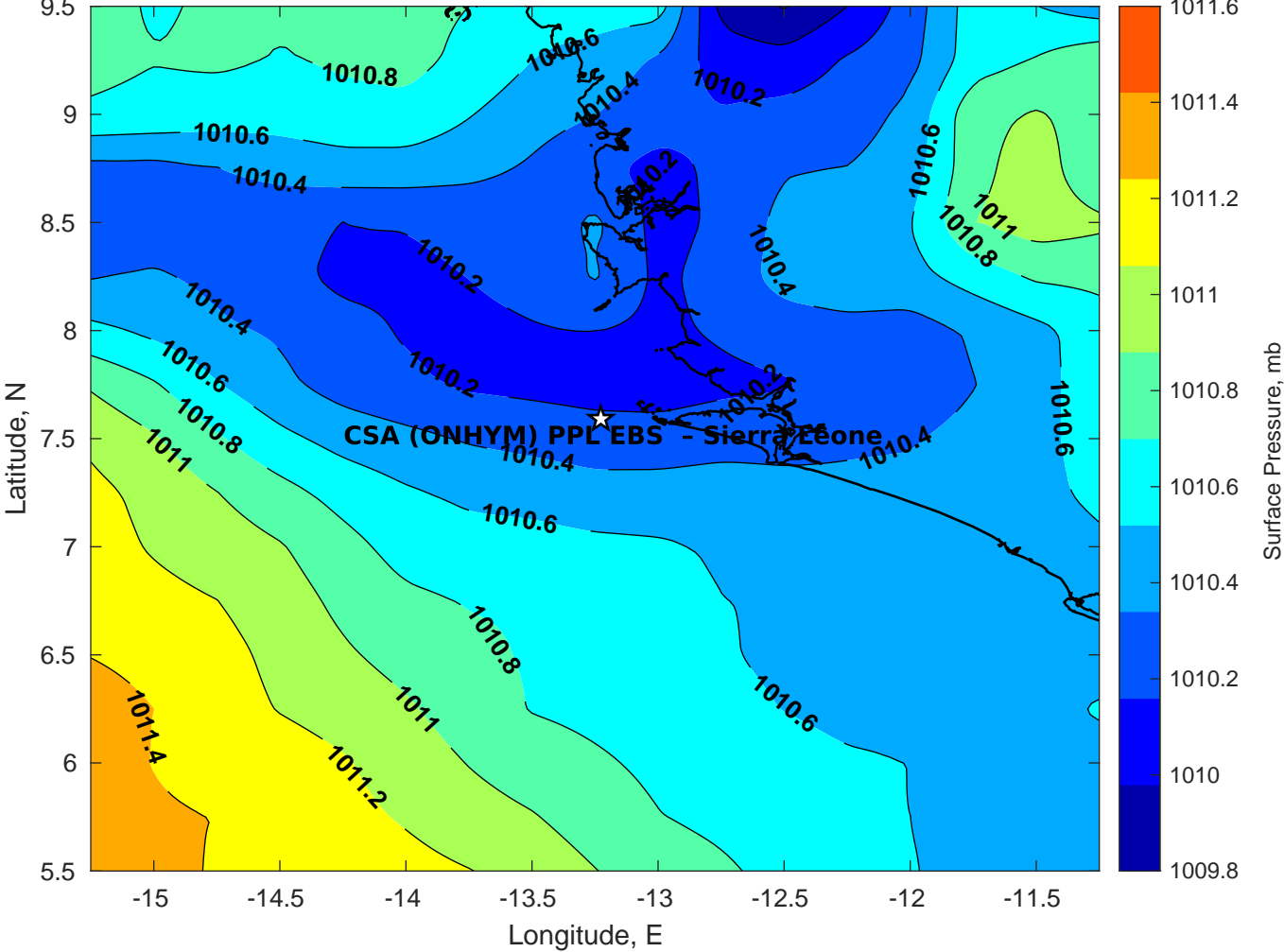
Surface Pressure (mb) for CSA (ONHYM) PPL EBS - Sierra Leone at 27-Mar-2025 00:00:00
