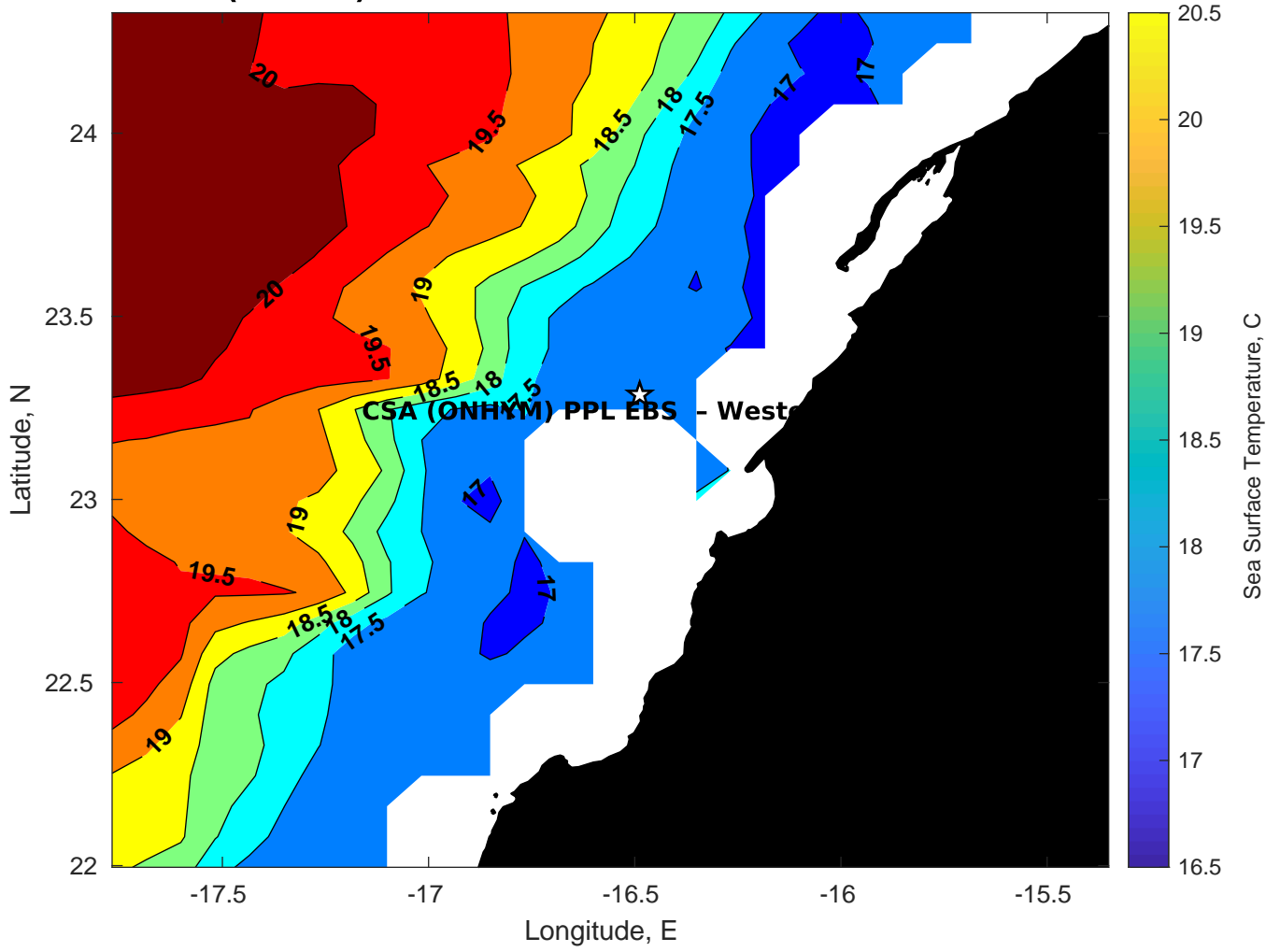
SST for CSA (ONHYM) PPL EBS - Western Sahara at 24-Mar-2025 00:00:00
