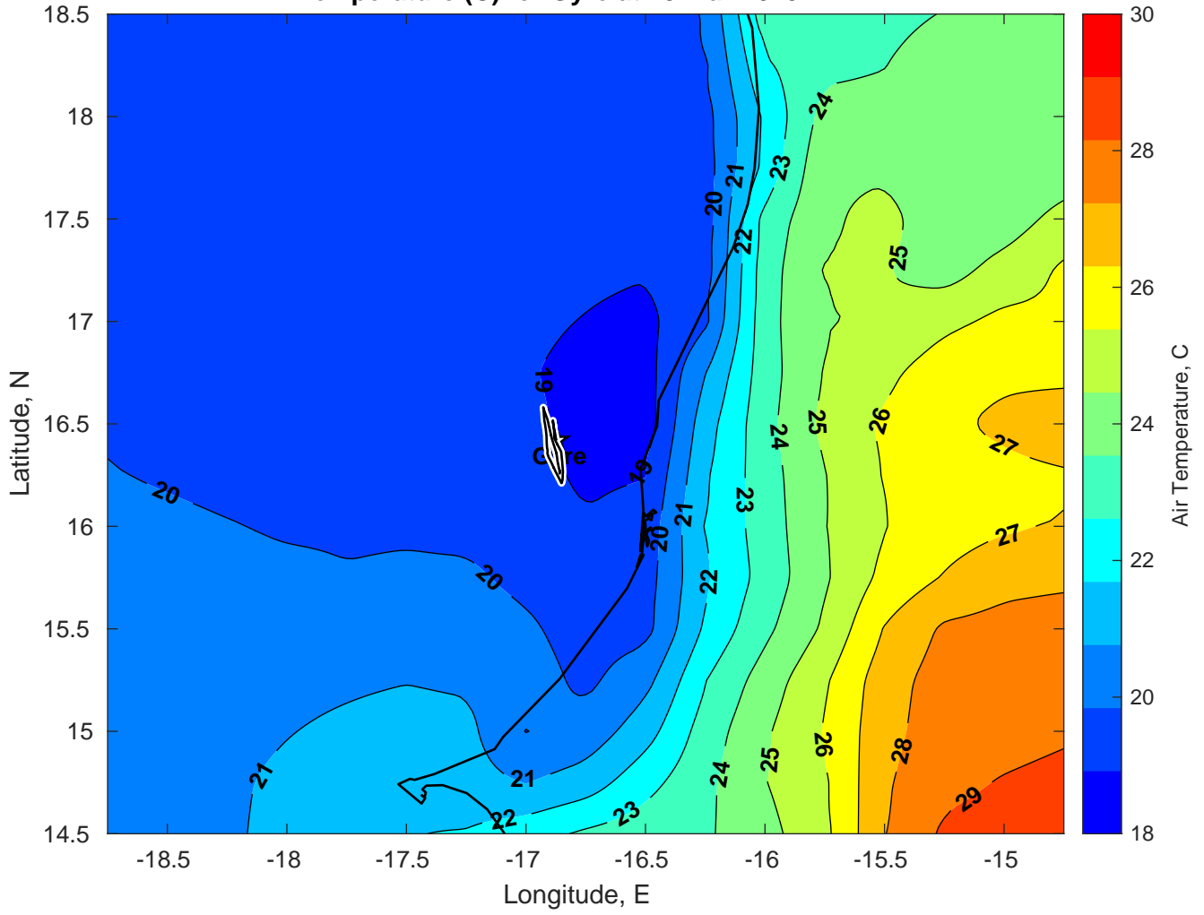
Air Temperature (C) for Gyre at 25-Mar-2025
