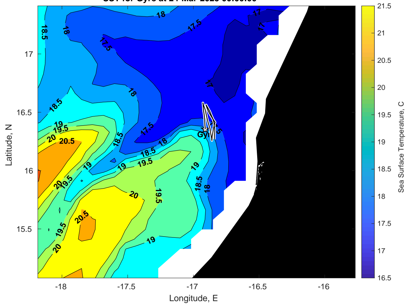
SST for Gyre at 24-Mar-2025 00:00:00
