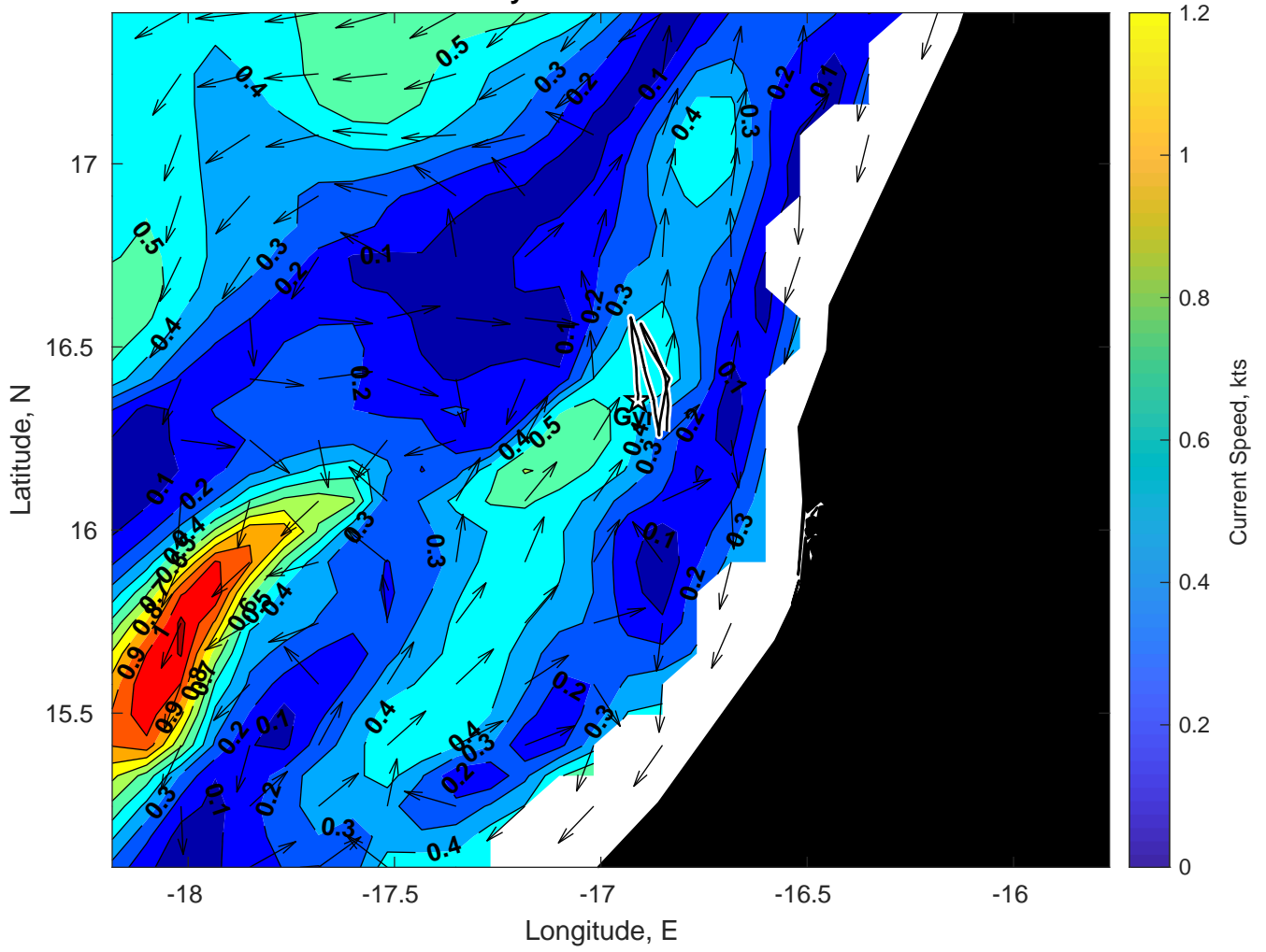
Surface Currents for Gyre at 24-Mar-2025 00:00:00
