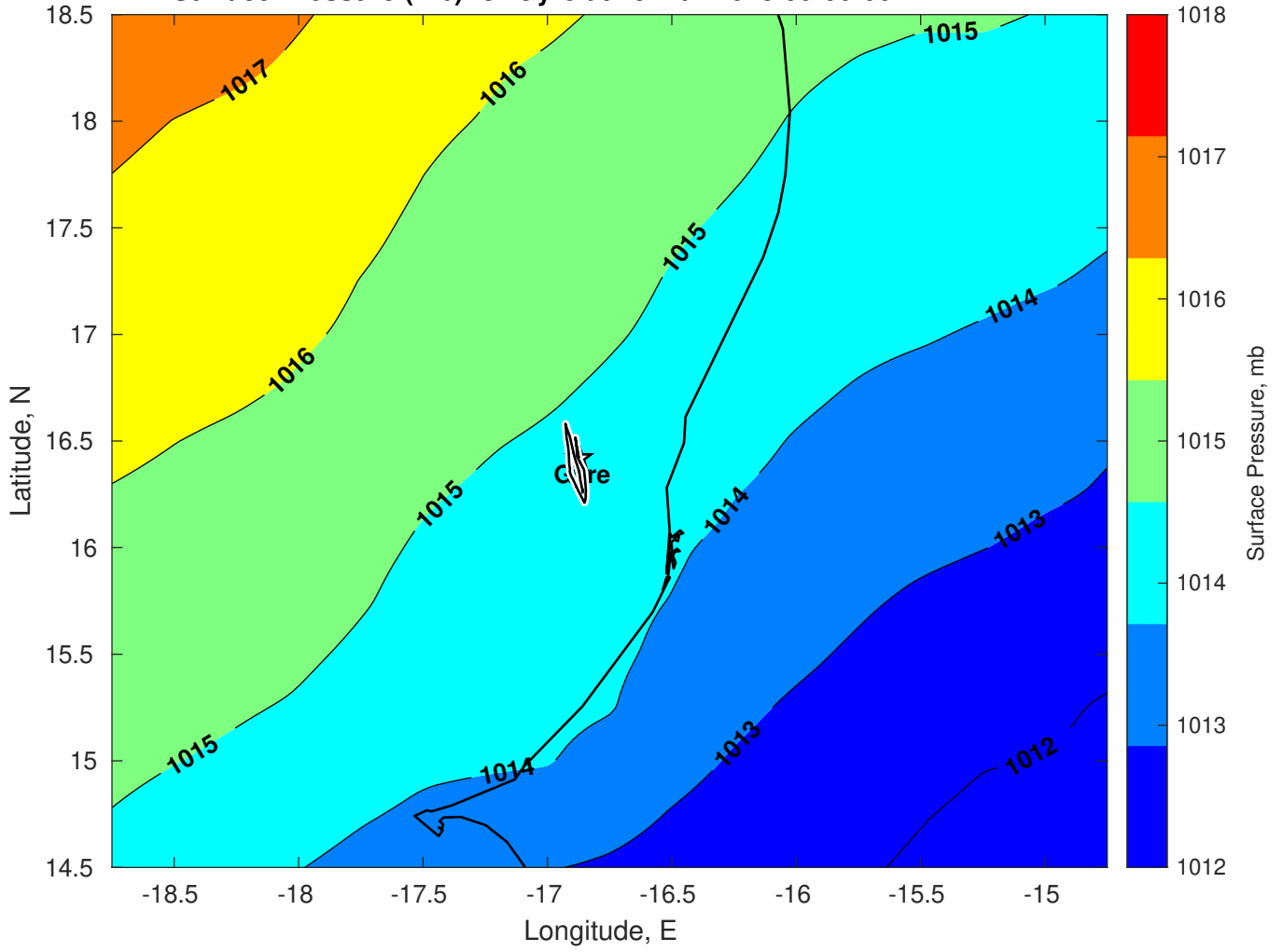
Surface Pressure (mb) for Gyre at 25-Mar-2025 00:00:00
