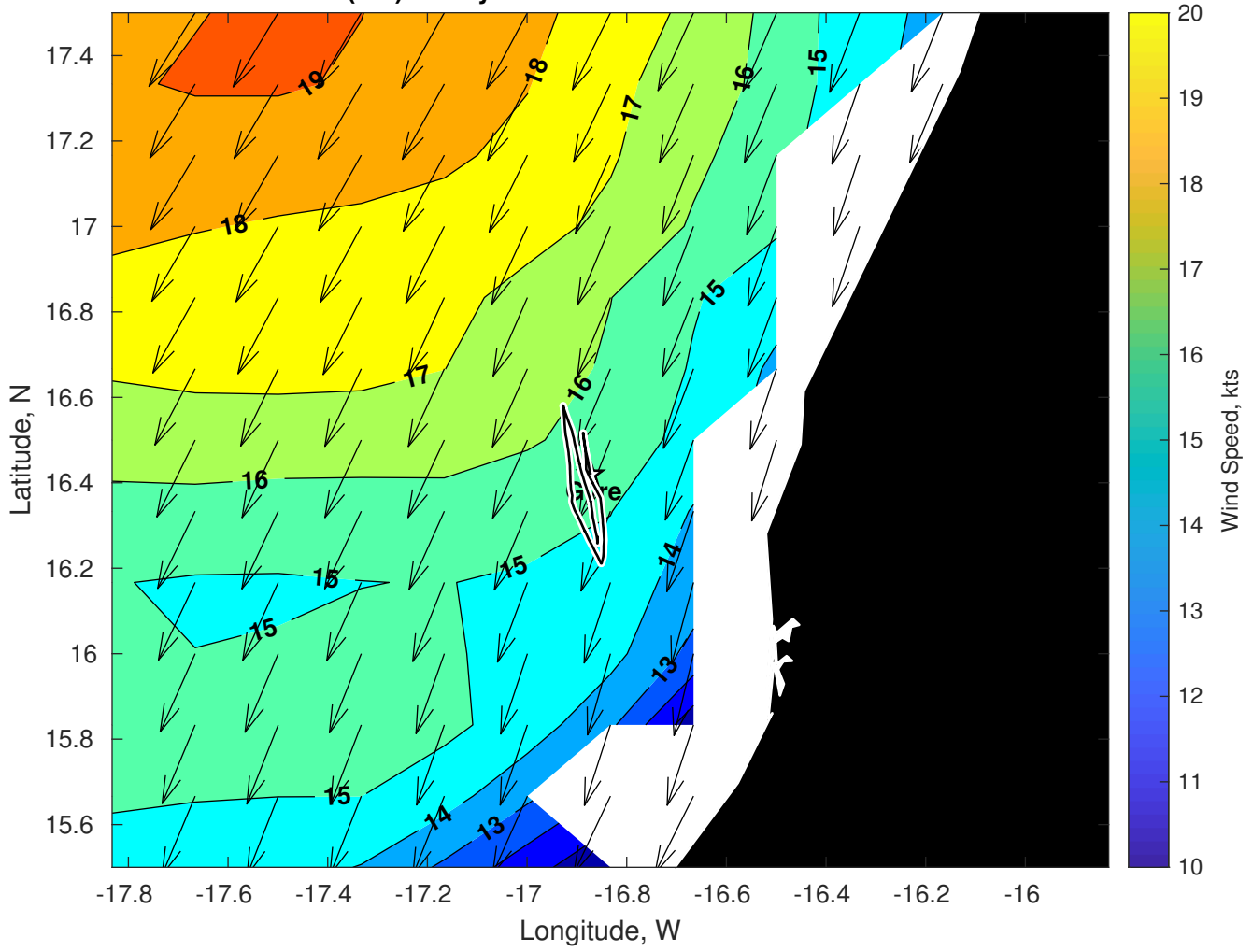
Winds (kts) for Gyre at 25-Mar-2025 09:00:00
