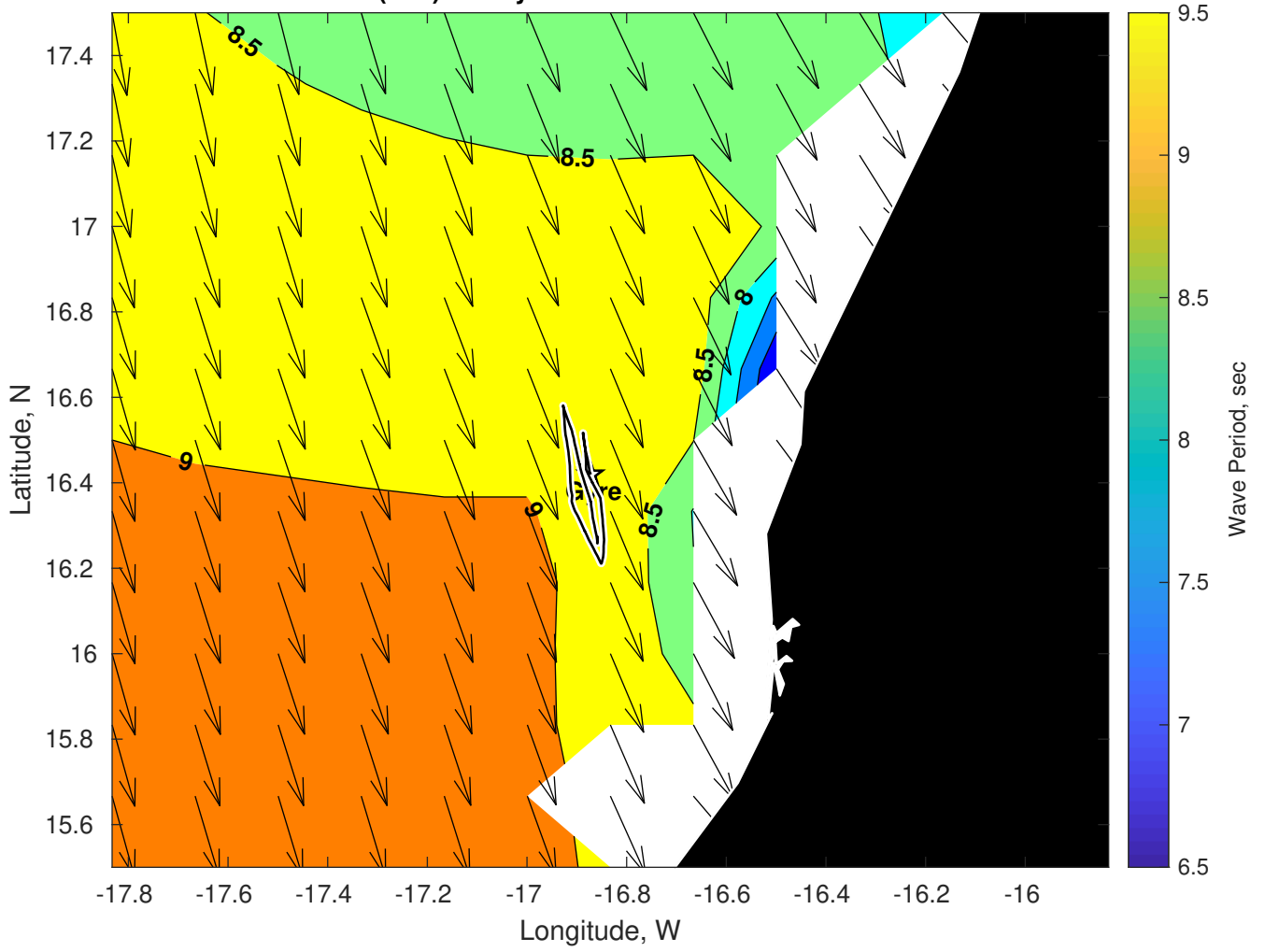
Wave Period (sec) for Gyre at 25-Mar-2025 09:00:00
