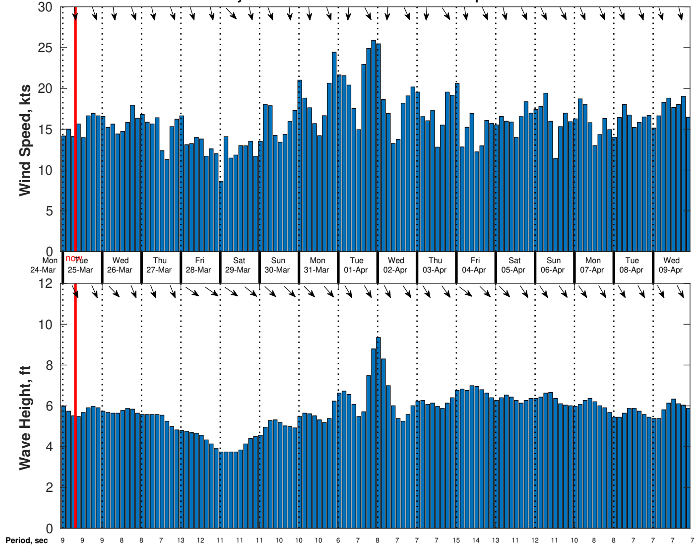
Wind & Wave Forecast for Gyre from 24-Mar-2025 23:00:00 to 09-Apr-2025 23:00:00
