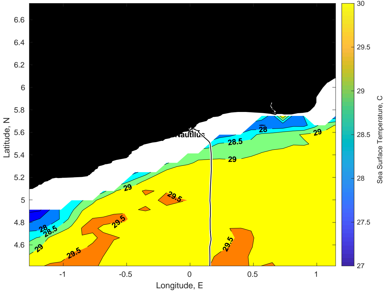
SST for Nautilus at 24-Mar-2025 00:00:00
