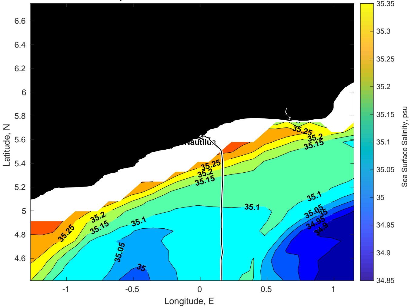
Surface Salinity for Nautilus at 24-Mar-2025 00:00:00
