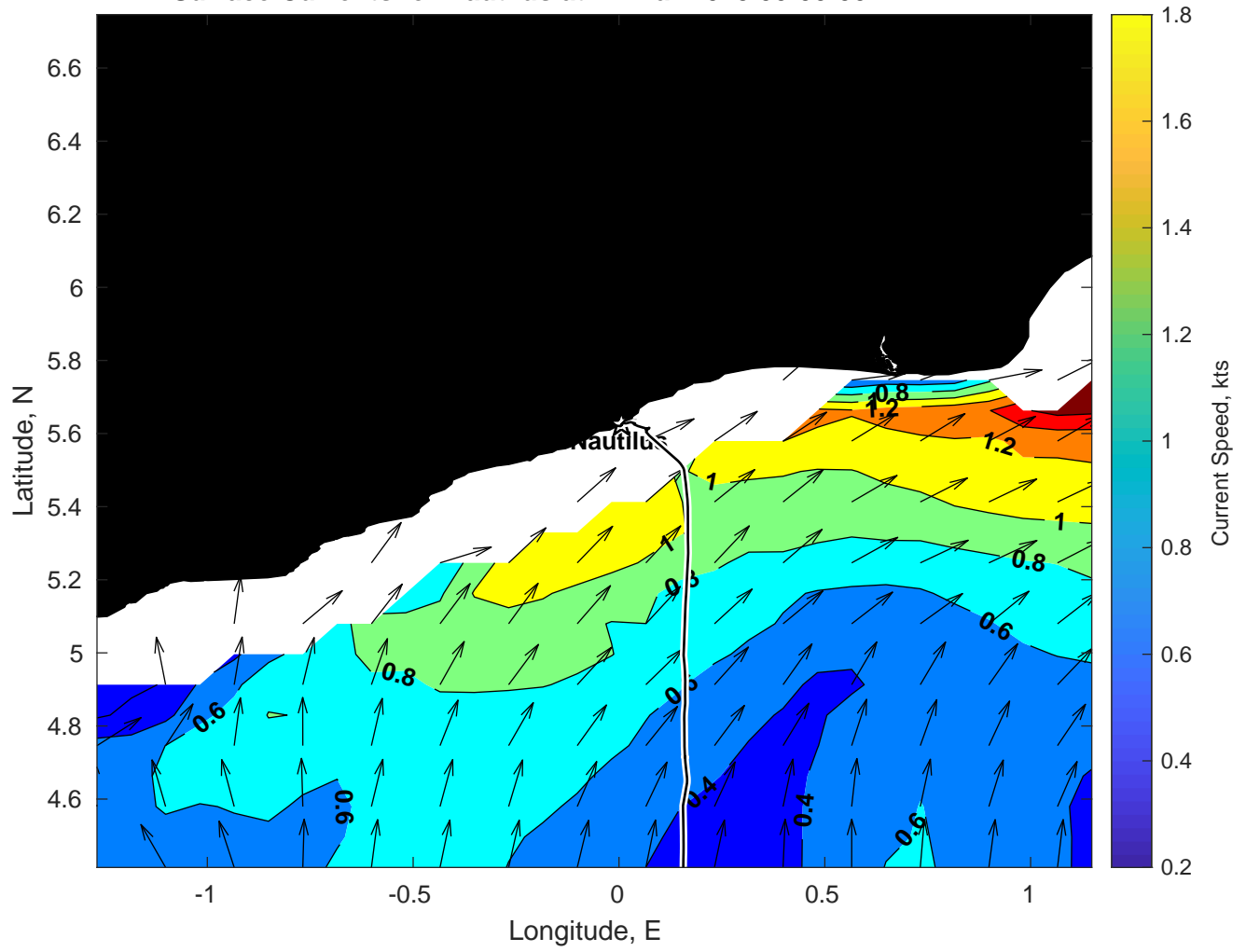
Surface Currents for Nautilus at 24-Mar-2025 00:00:00
