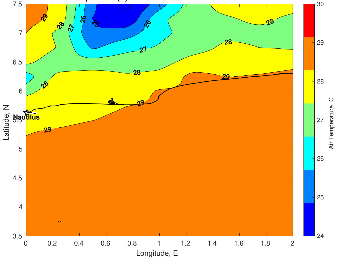
Air Temperature (C) for Nautilus at 25-Mar-2025
