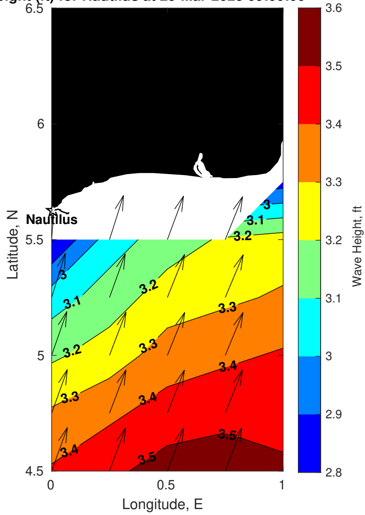
Wave Height (ft) for Nautilus at 25-Mar-2025 09:00:00
