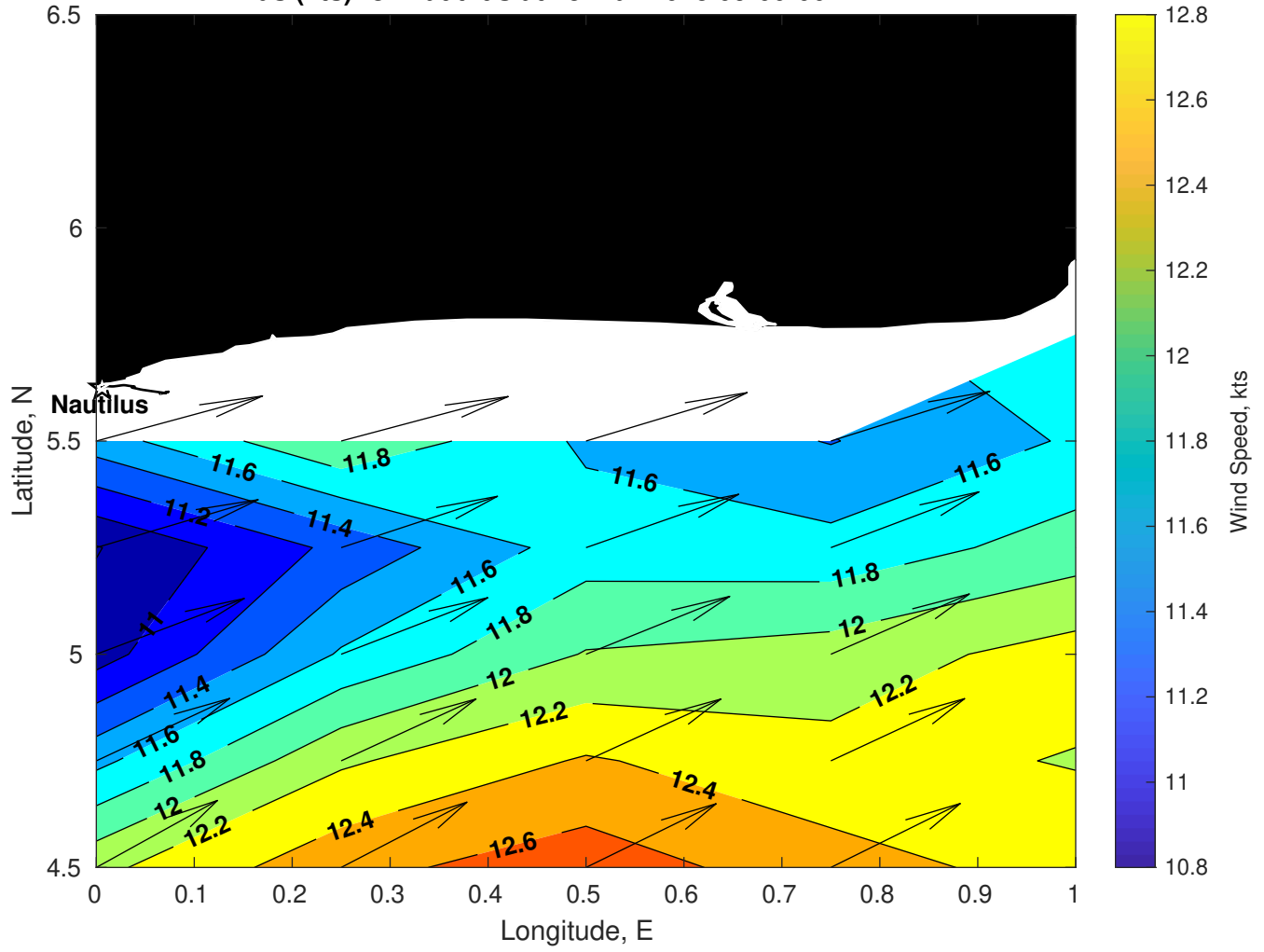
Winds (kts) for Nautilus at 25-Mar-2025 09:00:00
