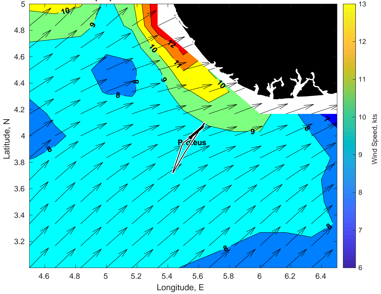
Winds (kts) for Proteus at 25-Mar-2025 09:00:00
