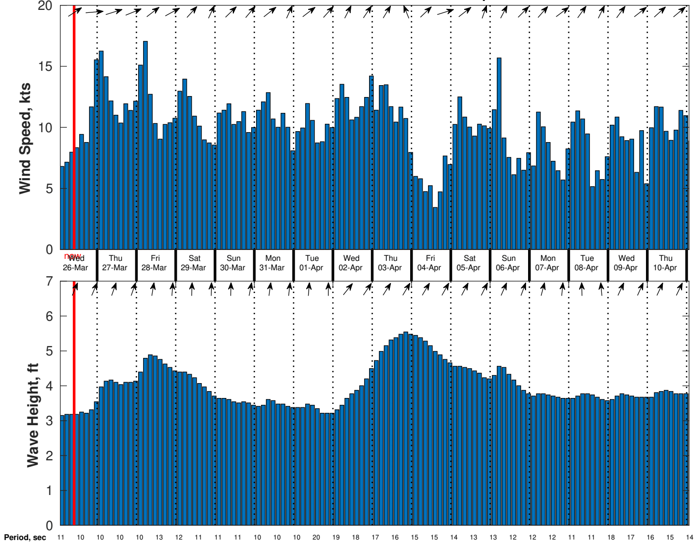
Wind & Wave Forecast for Proteus from 25-Mar-2025 01:00:00 to 10-Apr-2025 01:00:00
