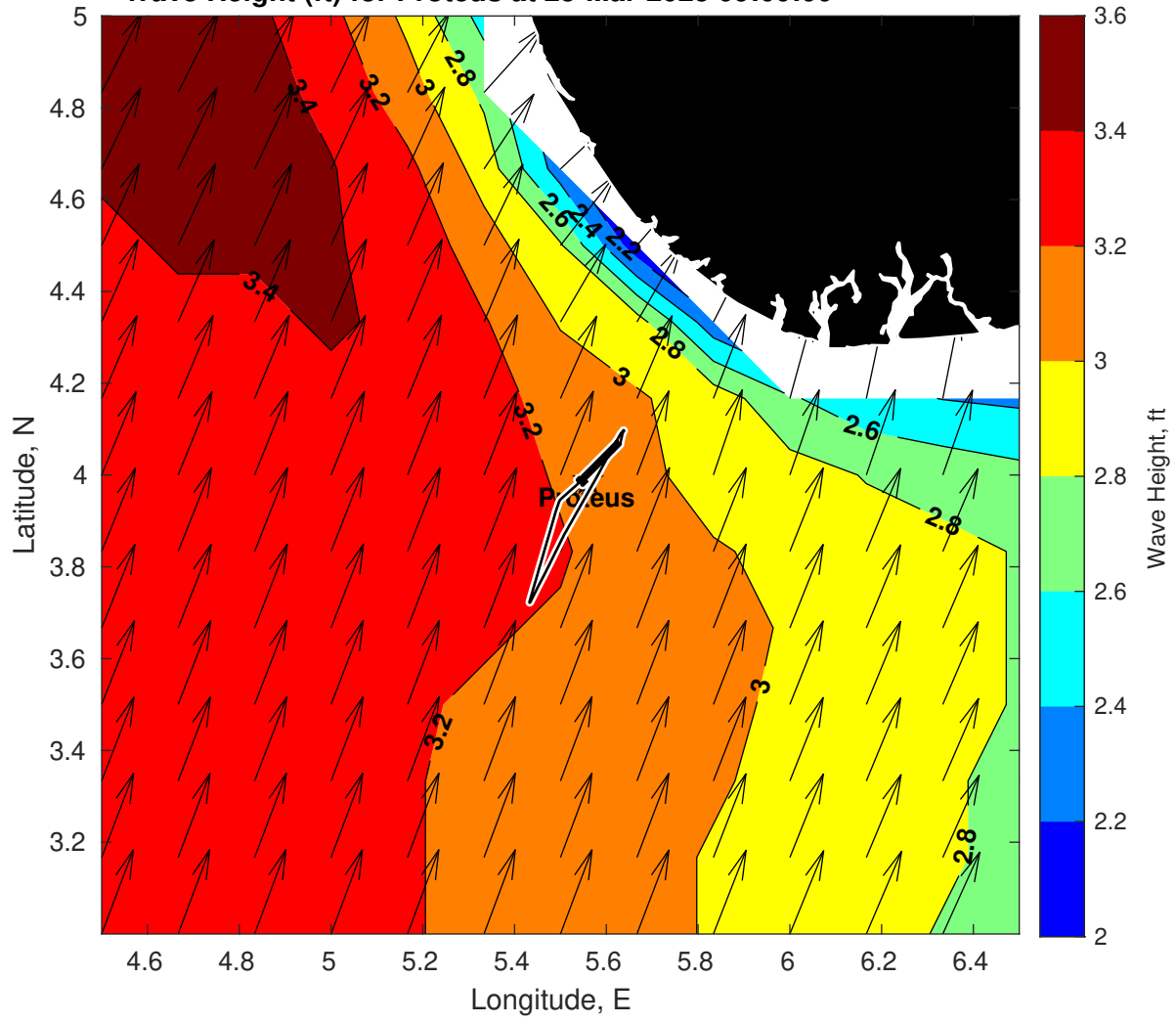
Wave Height (ft) for Proteus at 25-Mar-2025 09:00:00
