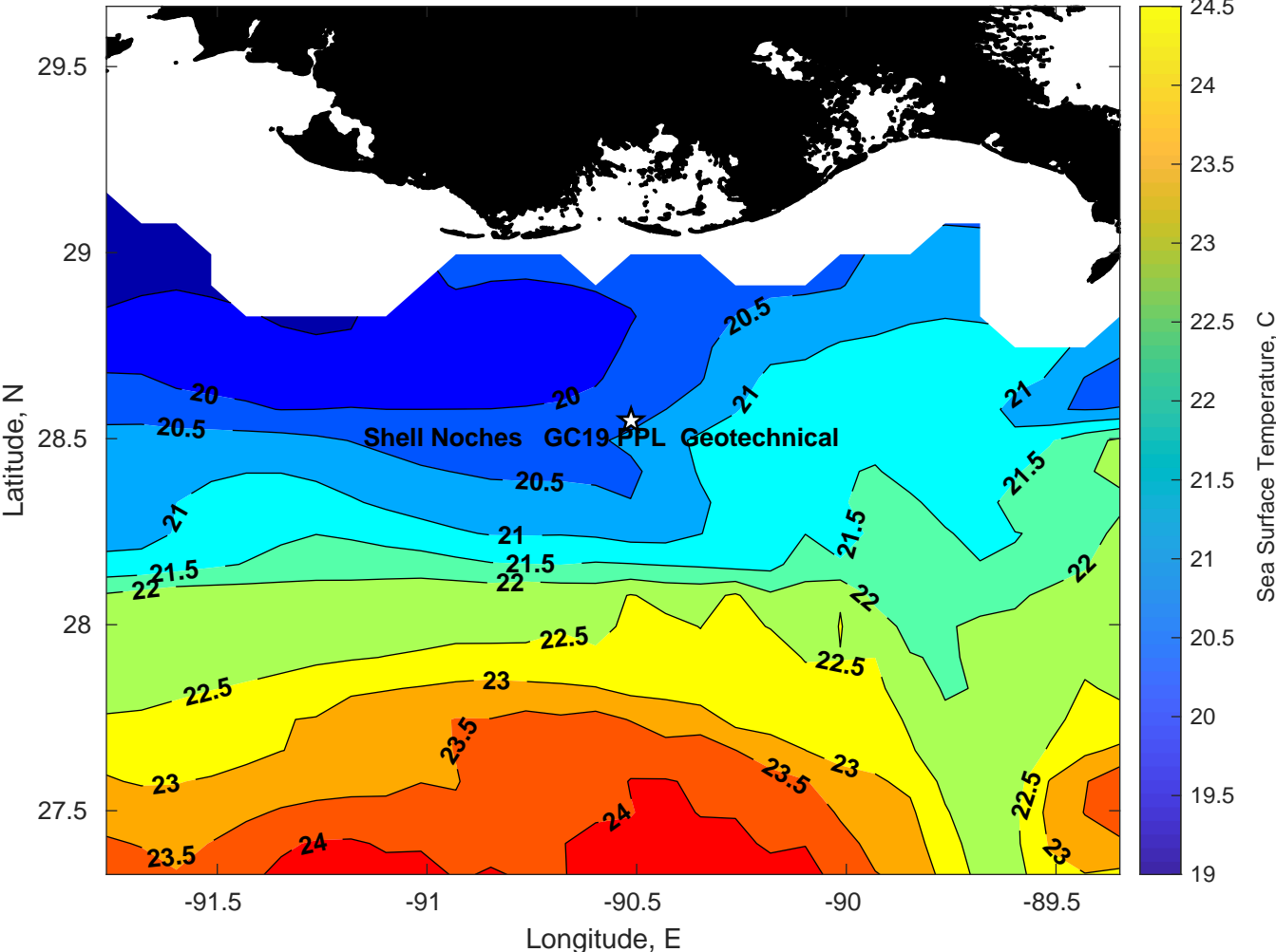
SST for Shell Noches GC19 PPL Geotechnical at 24-Mar-2025 00:00:00
