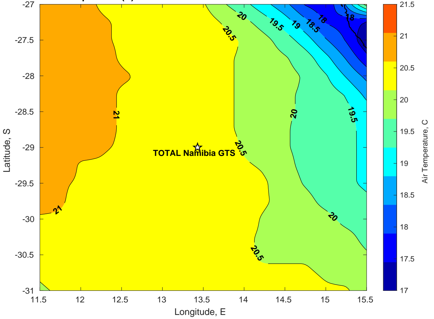
Air Temperature (C) for TOTAL Namibia GTS at 25-Mar-2025
