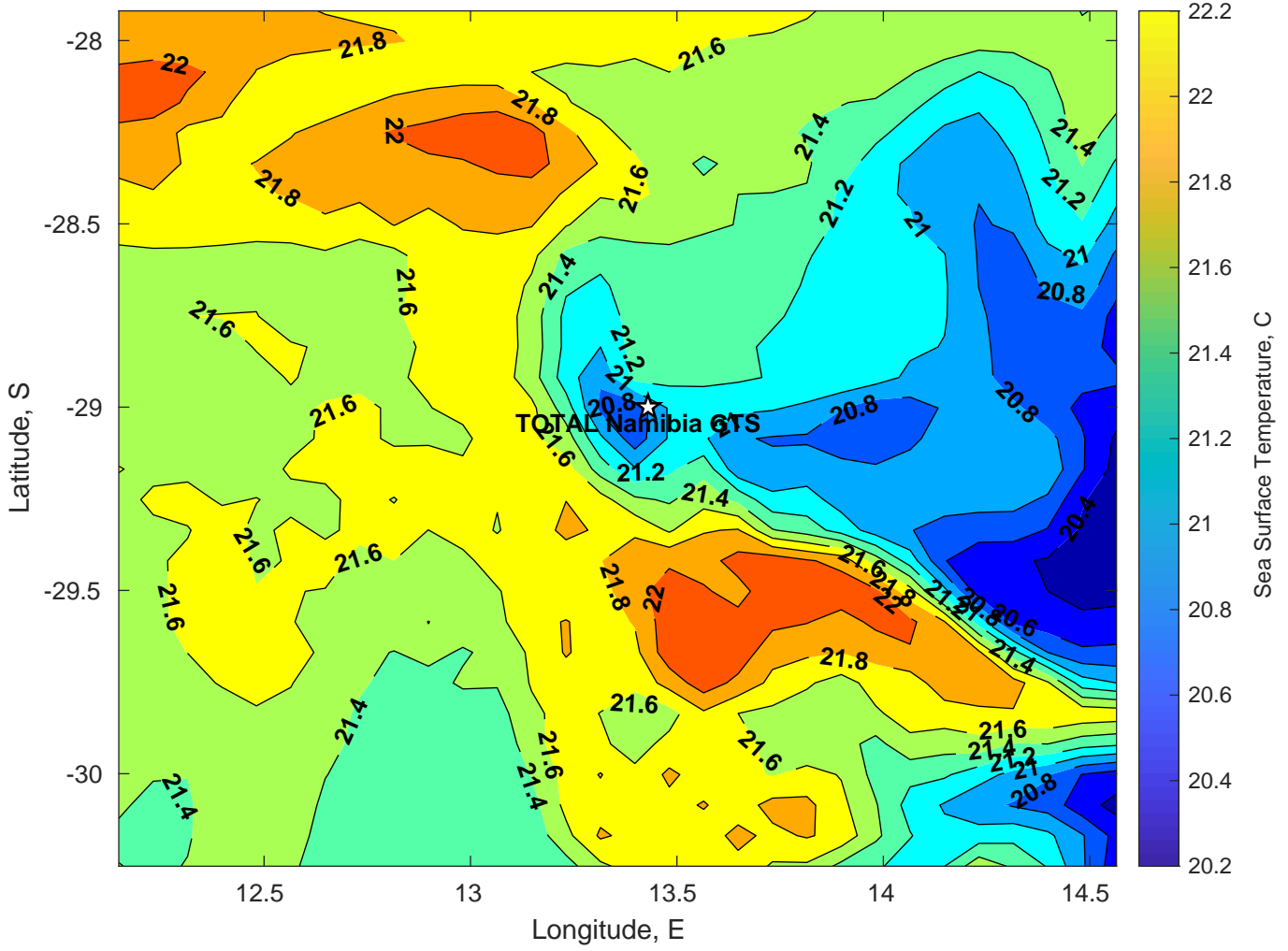
SST for TOTAL Namibia GTS at 24-Mar-2025 00:00:00
