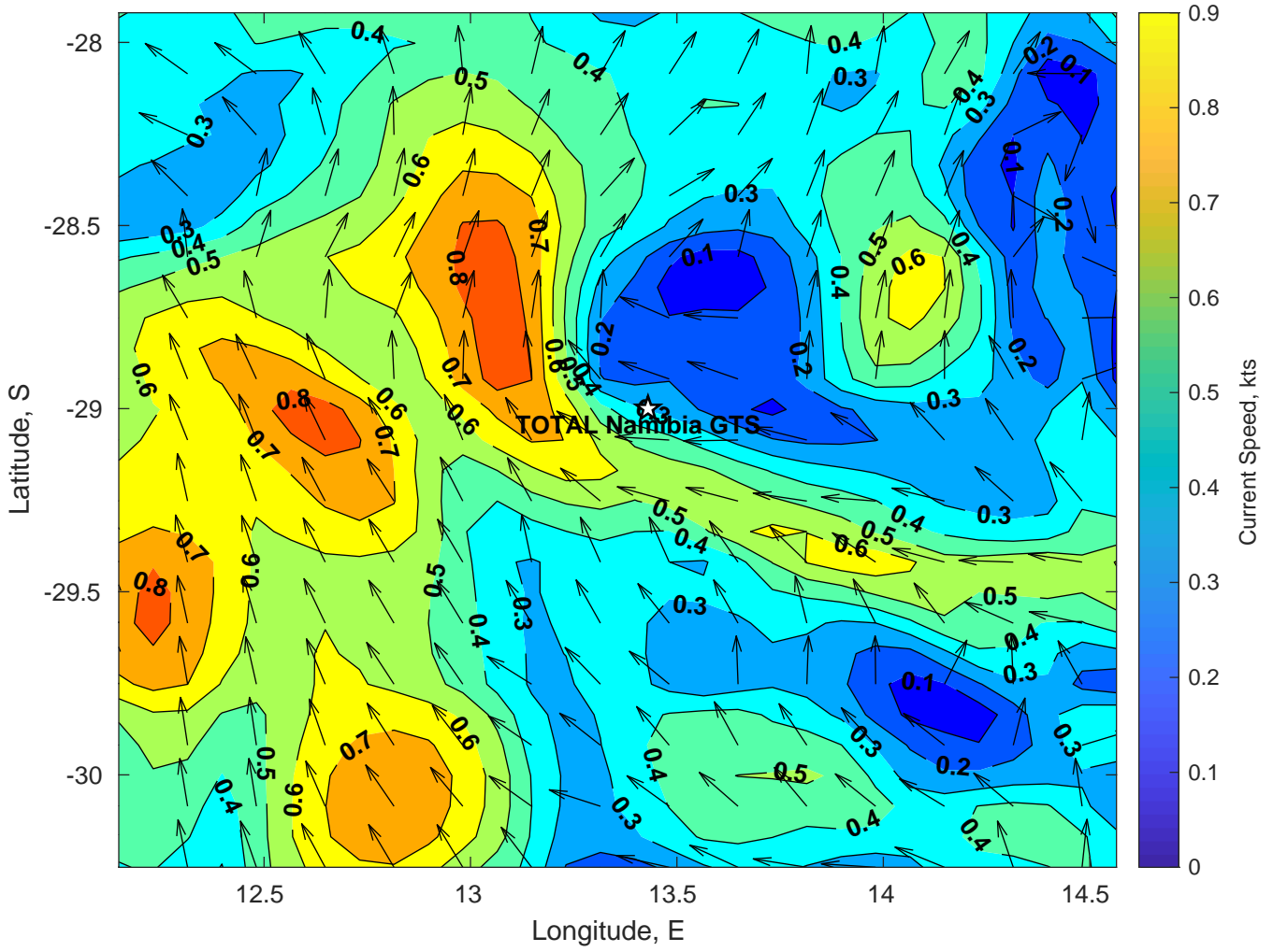
Surface Currents for TOTAL Namibia GTS at 24-Mar-2025 00:00:00
