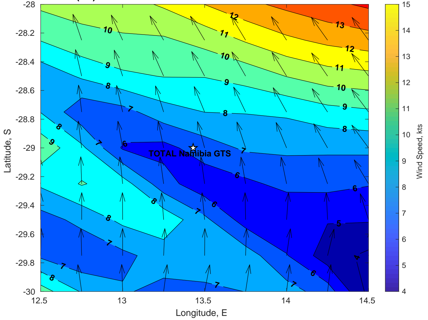
Winds (kts) for TOTAL Namibia GTS at 25-Mar-2025 09:00:00
