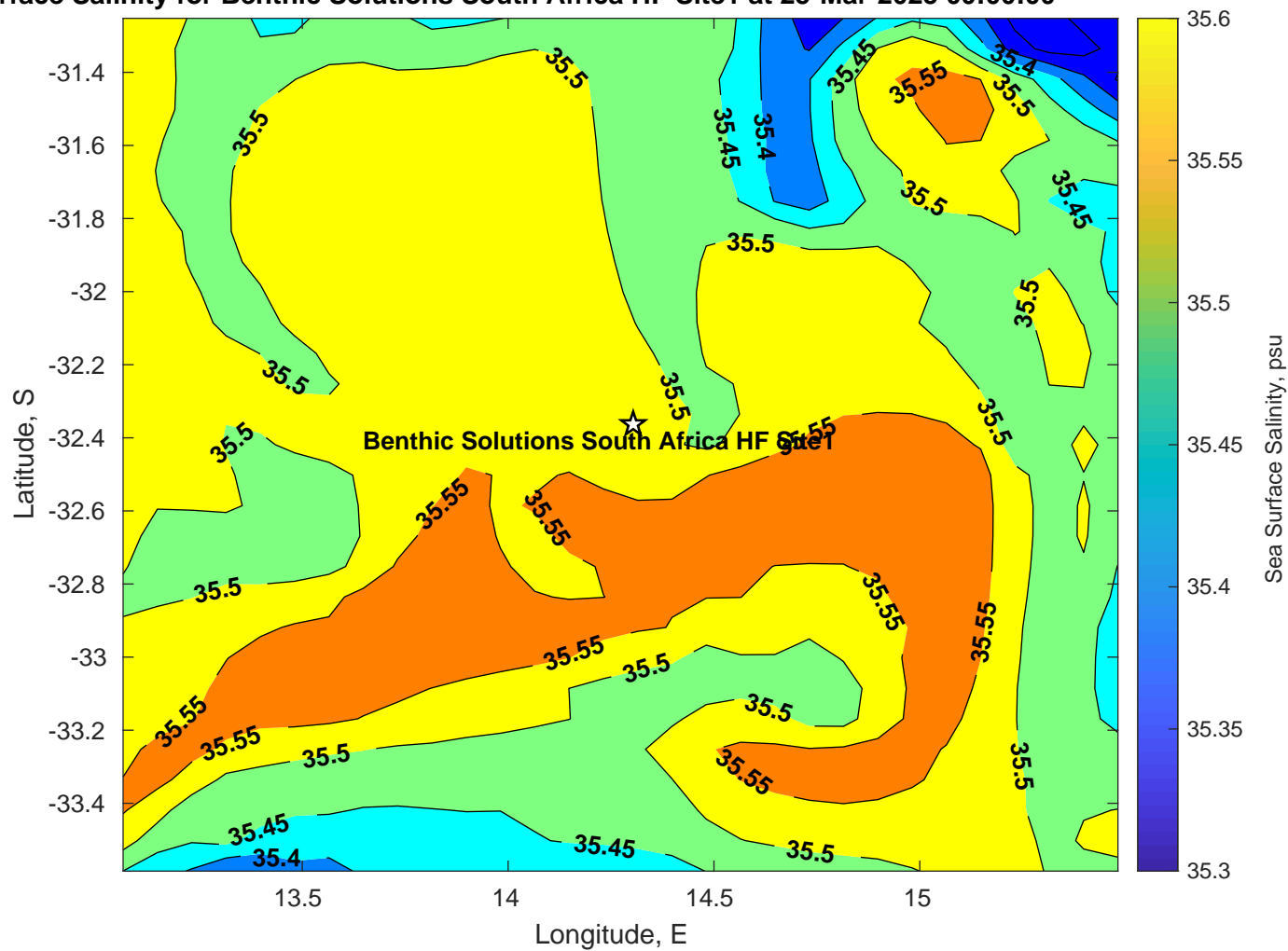
Surface Salinity for Benthic Solutions South Africa HF Site1 at 25-Mar-2025 00:00:00
