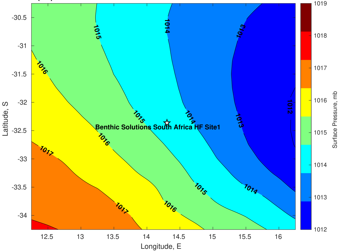
Surface Pressure (mb) for Benthic Solutions South Africa HF Site1 at 28-Mar-2025 00:00:00
