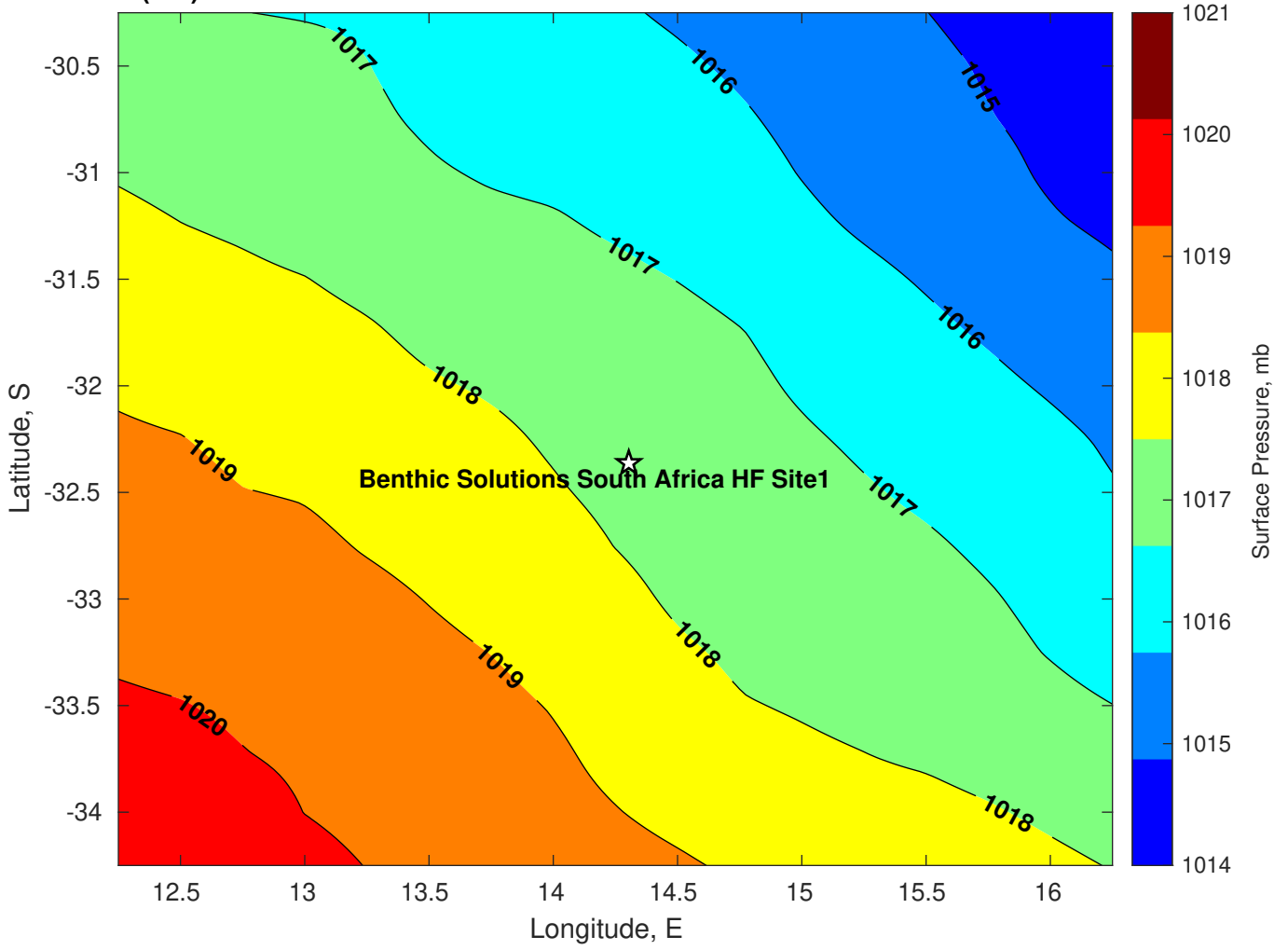
Surface Pressure (mb) for Benthic Solutions South Africa HF Site1 at 27-Mar-2025 00:00:00
