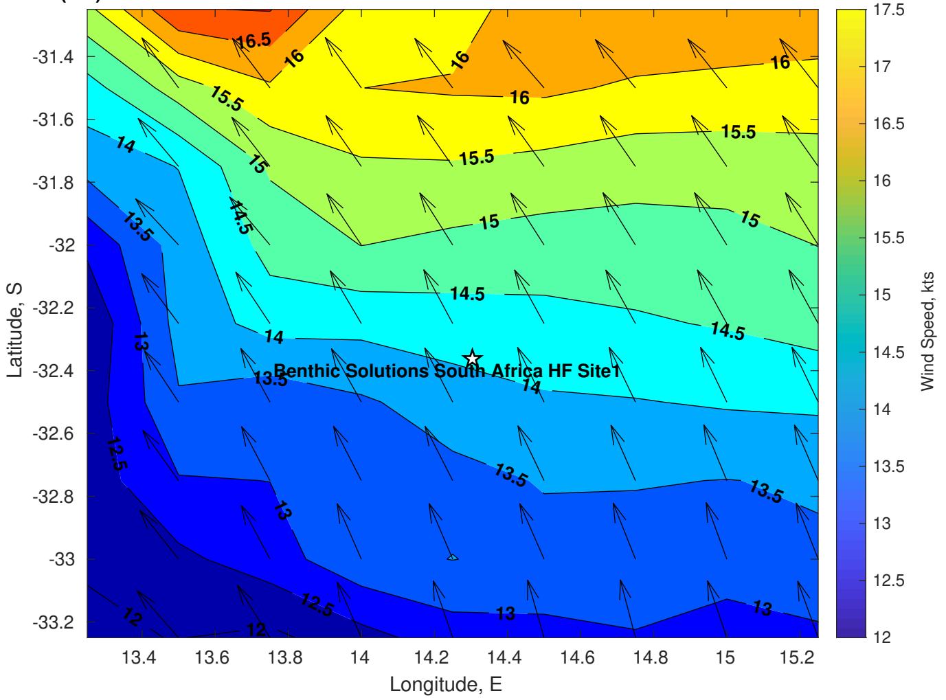
Winds (kts) for Benthic Solutions South Africa HF Site1 at 26-Mar-2025 09:00:00
