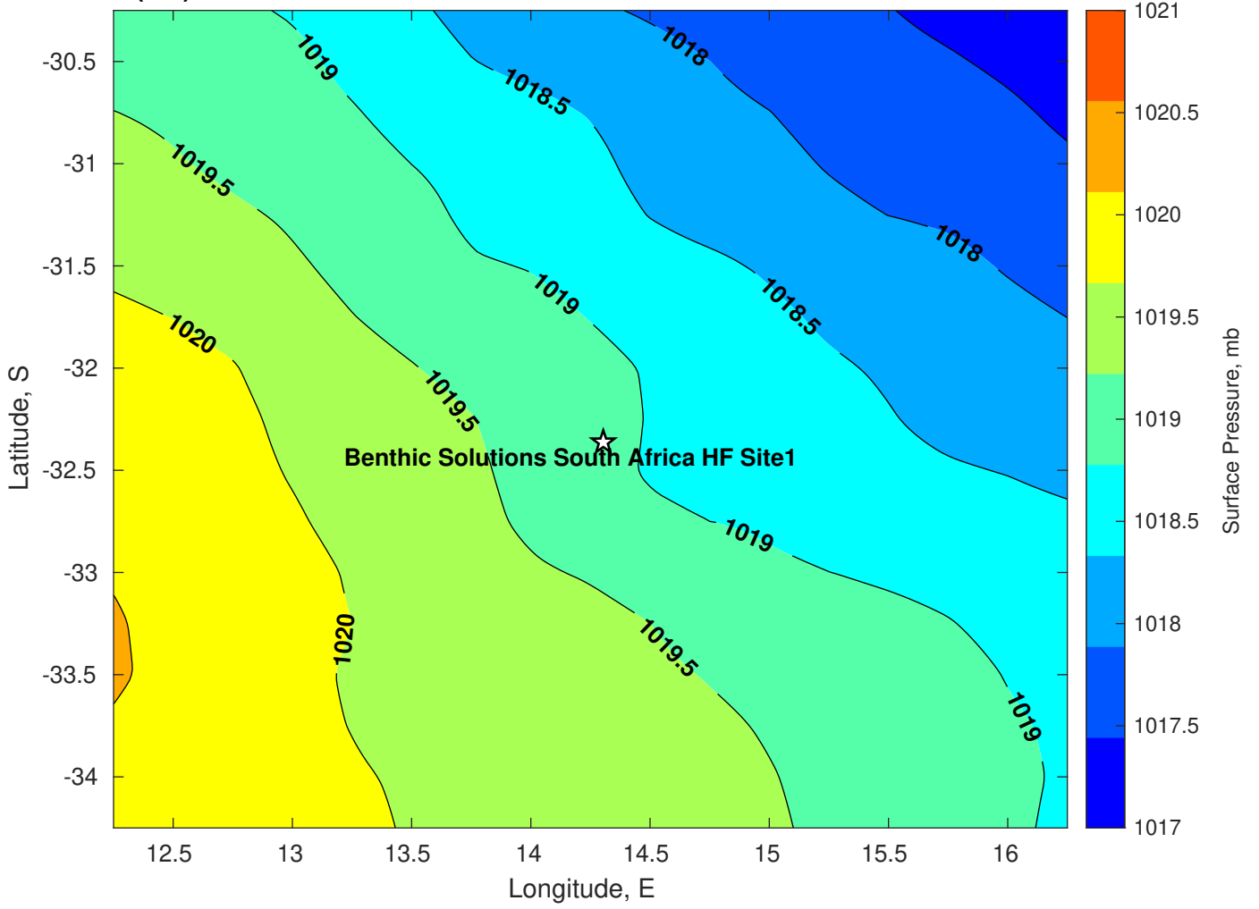
Surface Pressure (mb) for Benthic Solutions South Africa HF Site1 at 26-Mar-2025 00:00:00
