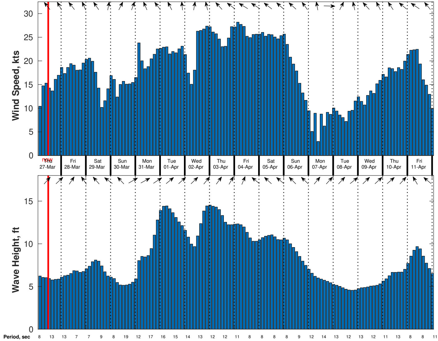
Wind & Wave Forecast for Benthic Solutions South Africa HF Site1 from 26-Mar-2025 02:00:00 to 11-Apr-2025 02:00:00
