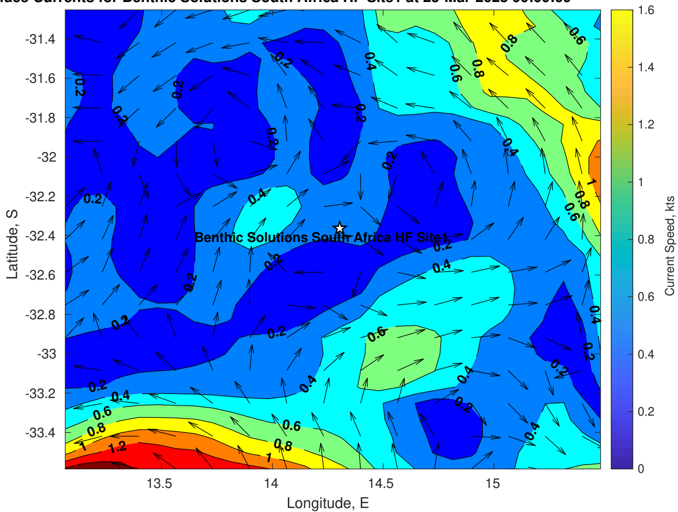
Surface Currents for Benthic Solutions South Africa HF Site1 at 25-Mar-2025 00:00:00
