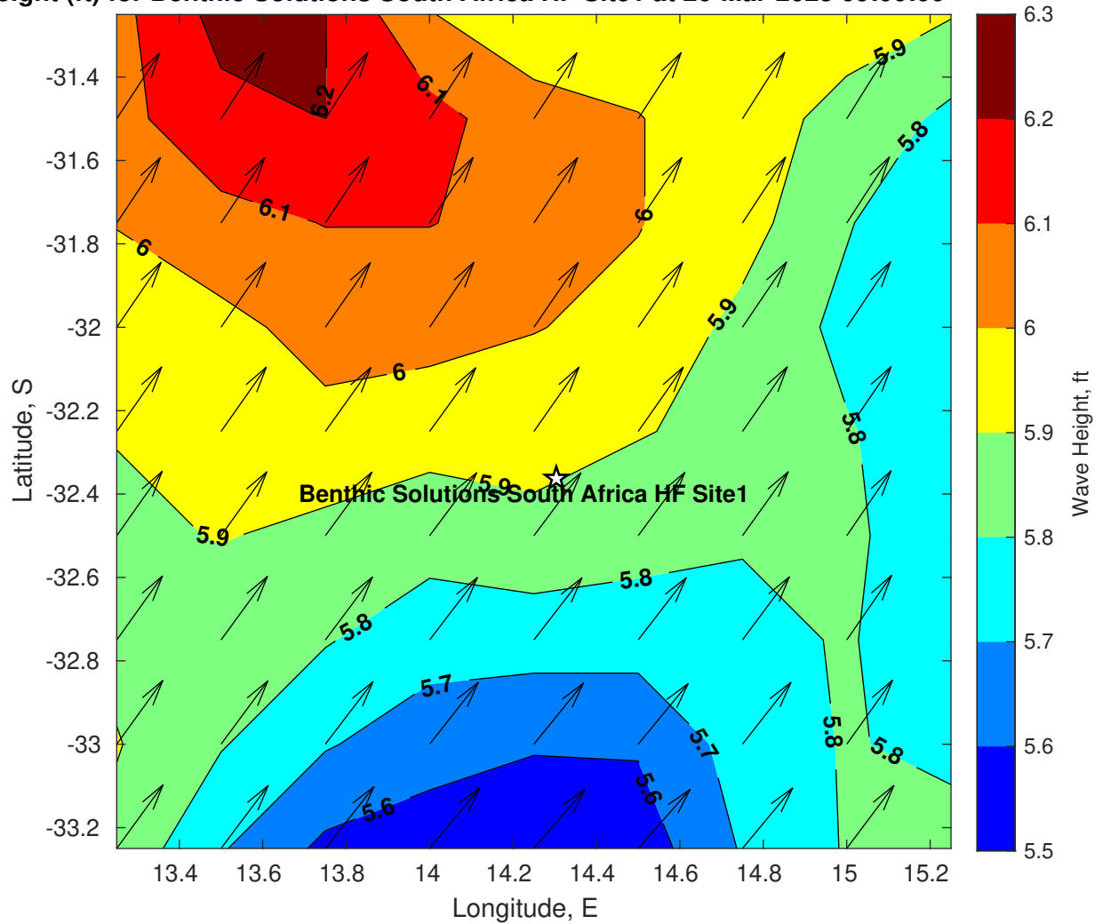
Wave Height (ft) for Benthic Solutions South Africa HF Site1 at 26-Mar-2025 09:00:00
