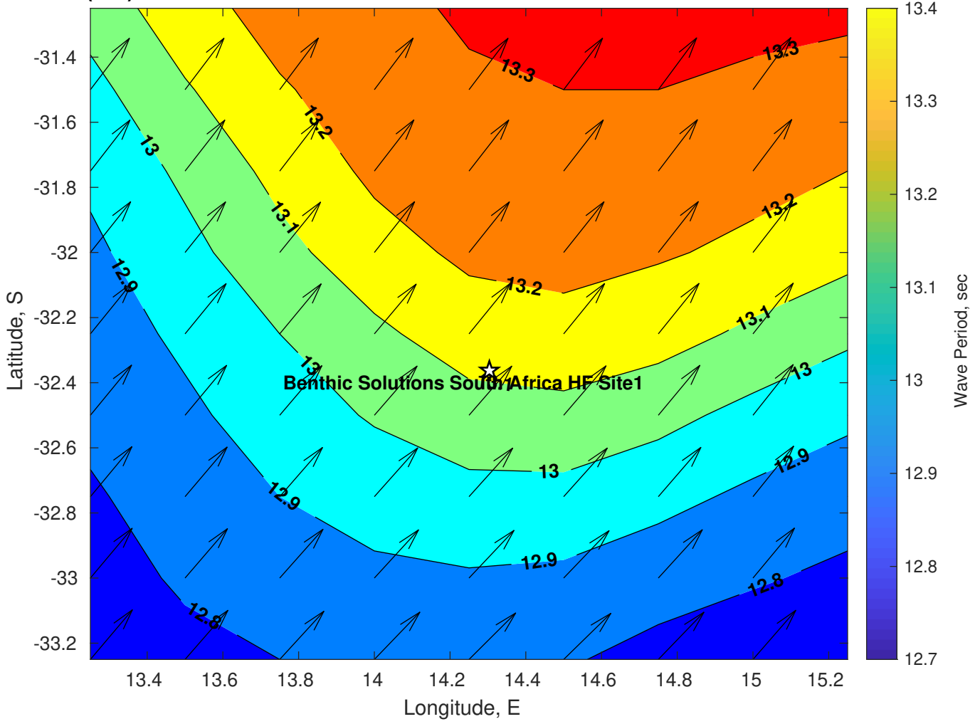
Wave Period (sec) for Benthic Solutions South Africa HF Site1 at 26-Mar-2025 09:00:00
