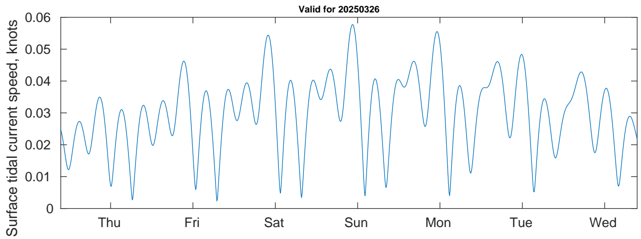
Tidal Currents and Heights for Benthic Solutions South Africa HF Site1 at 20250326
