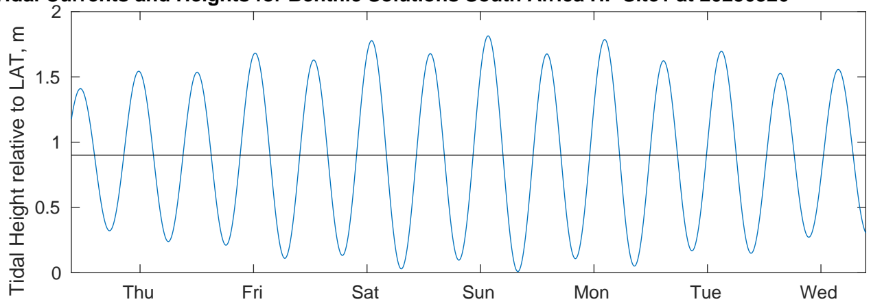
Tidal Currents and Heights for Benthic Solutions South Africa HF Site1 at 20250326
