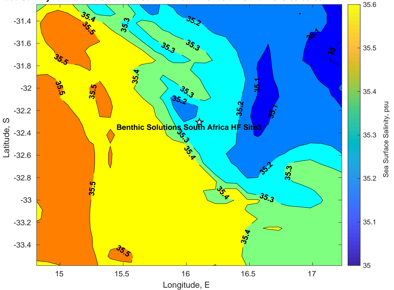
Surface Salinity for Benthic Solutions South Africa HF Site3 at 25-Mar-2025 00:00:00
