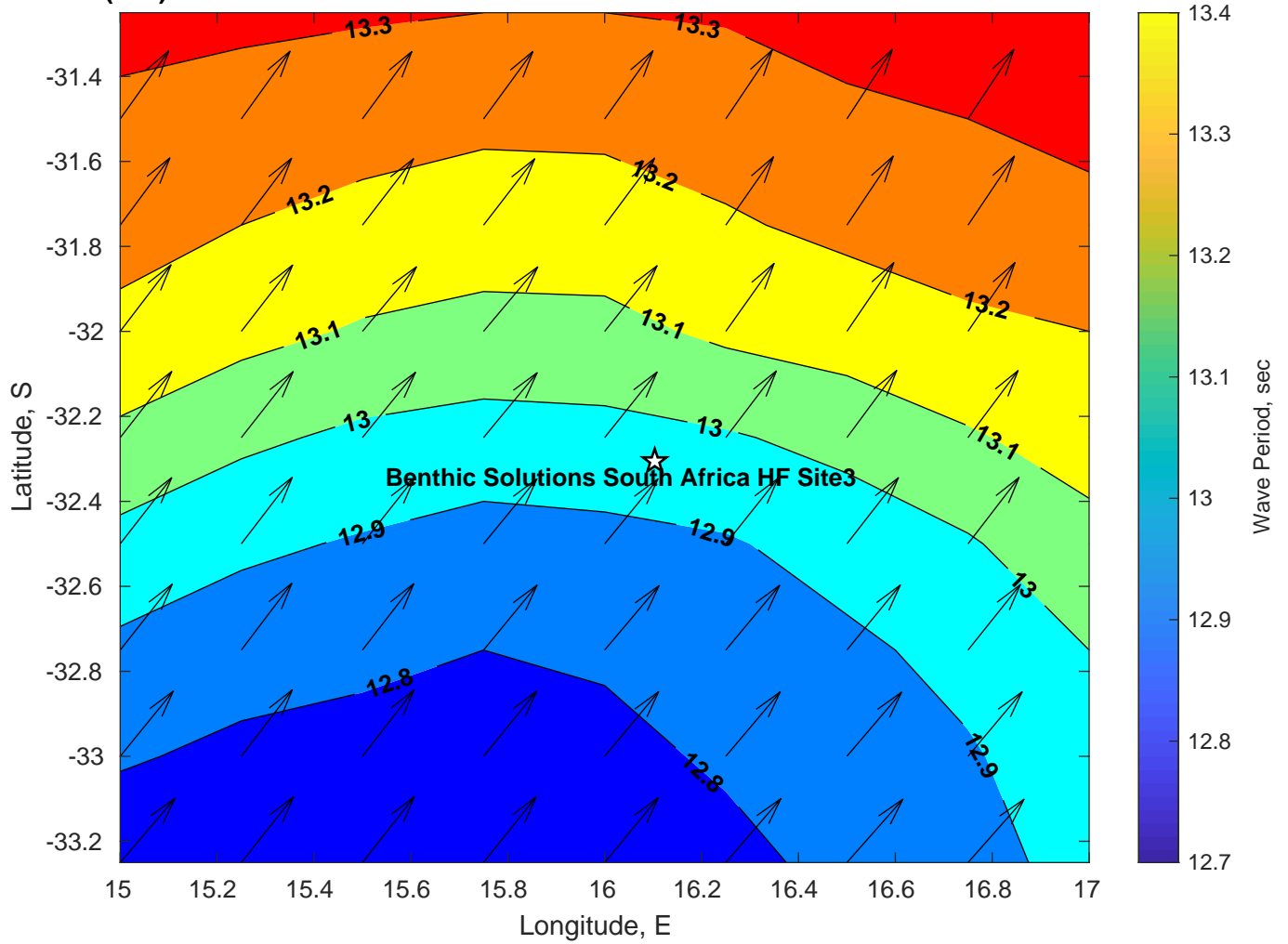
Wave Period (sec) for Benthic Solutions South Africa HF Site3 at 26-Mar-2025 09:00:00
