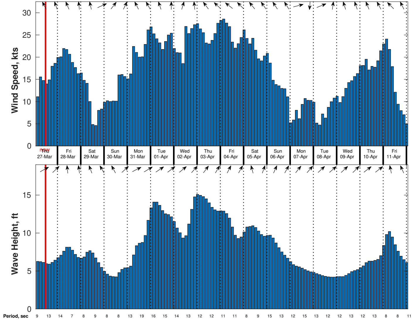
Wind & Wave Forecast for Benthic Solutions South Africa HF Site3 from 26-Mar-2025 02:00:00 to 11-Apr-2025 02:00:00
