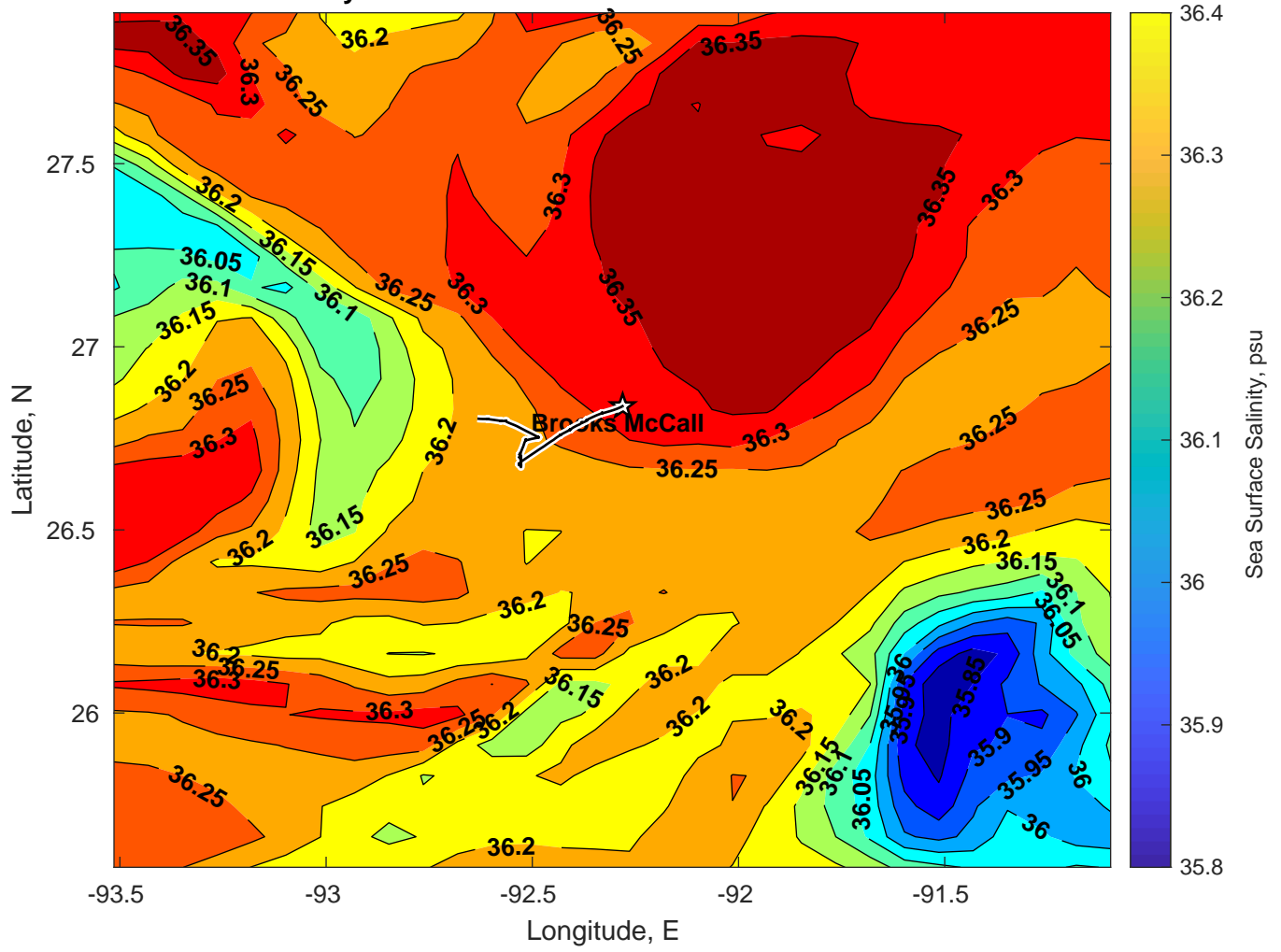
Surface Salinity for Brooks McCall at 25-Mar-2025 00:00:00
