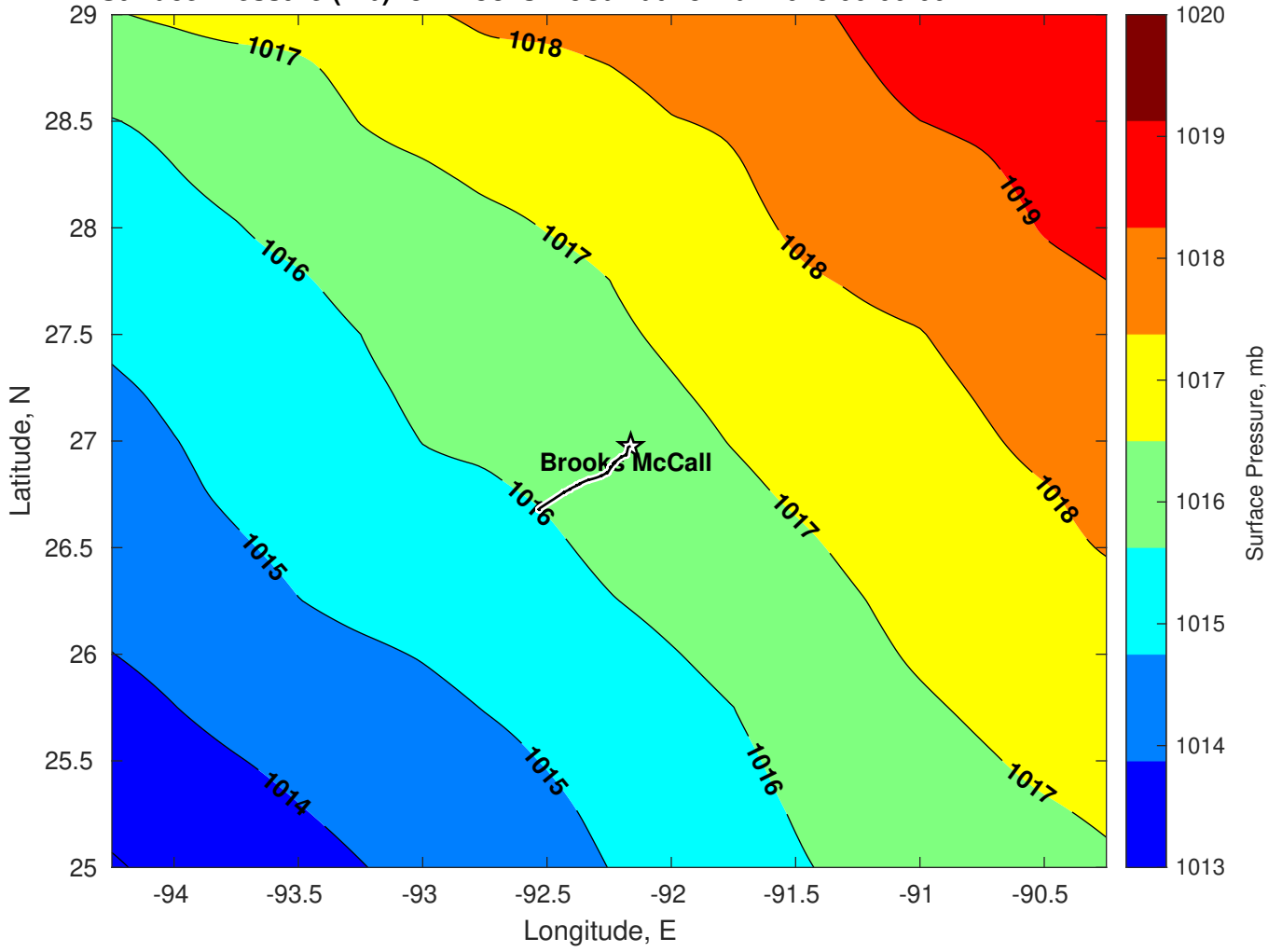
Surface Pressure (mb) for Brooks McCall at 28-Mar-2025 00:00:00
