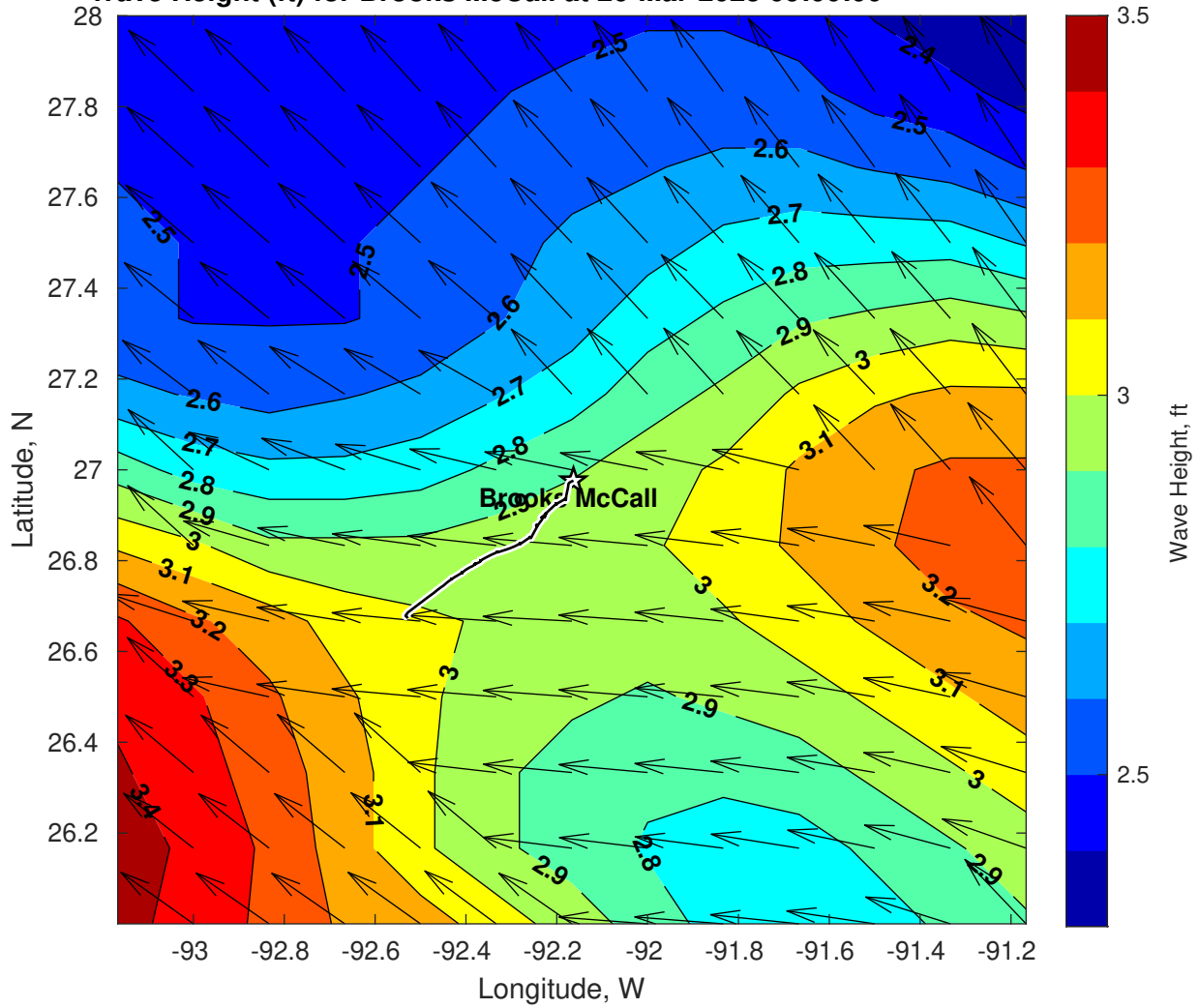
Wave Height (ft) for Brooks McCall at 26-Mar-2025 09:00:00
