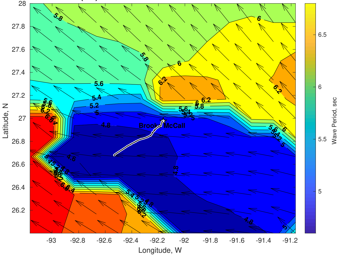
Wave Period (sec) for Brooks McCall at 26-Mar-2025 09:00:00
