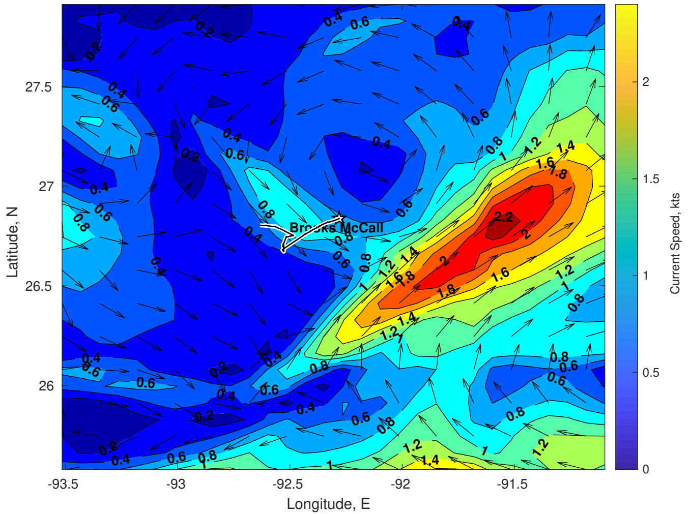
Surface Currents for Brooks McCall at 25-Mar-2025 00:00:00
