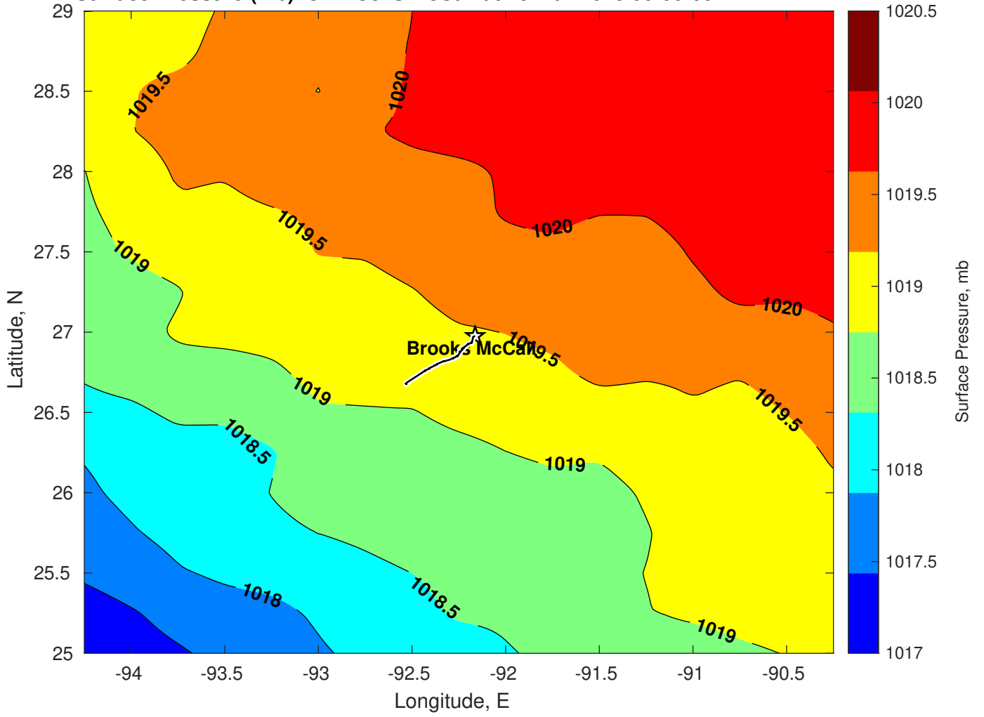
Surface Pressure (mb) for Brooks McCall at 26-Mar-2025 00:00:00
