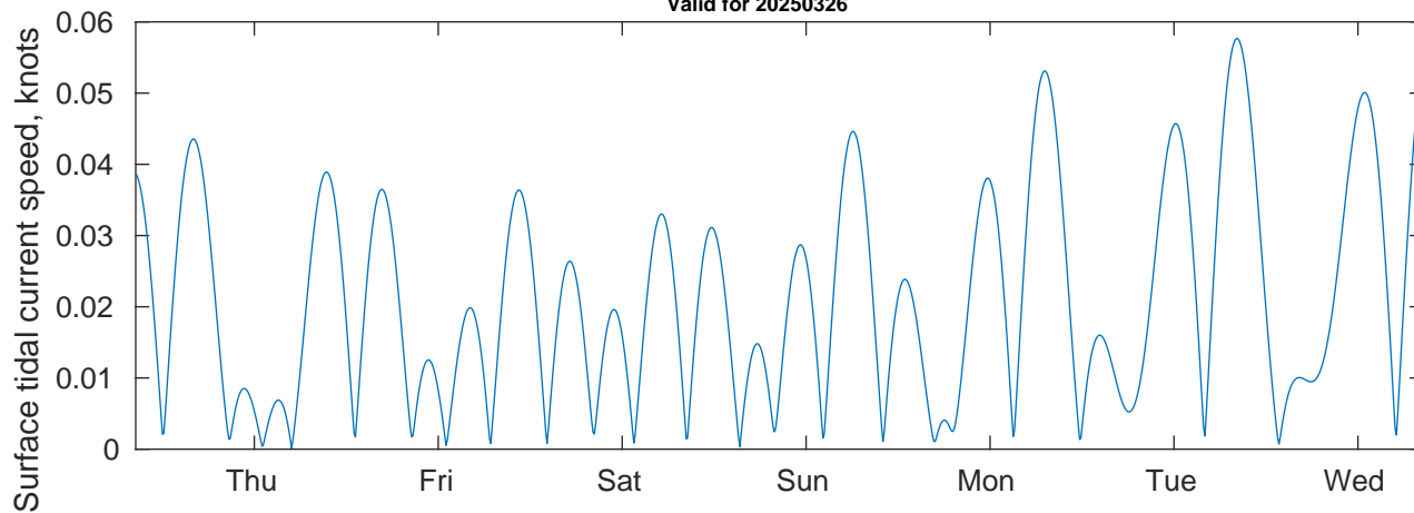
Tidal Currents and Heights for Brooks McCall at 20250326
