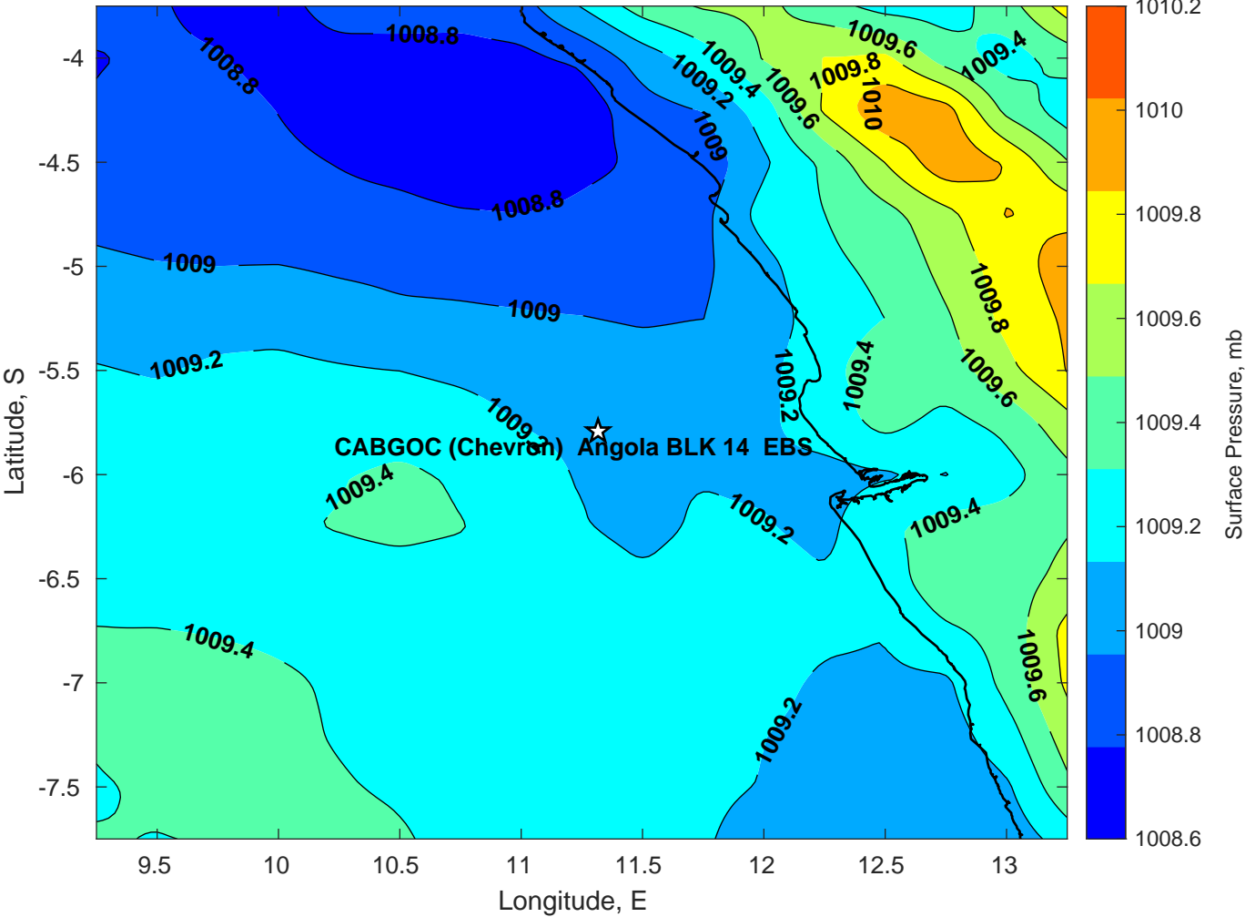
Surface Pressure (mb) for CABGOC (Chevron) Angola BLK 14 EBS at 28-Mar-2025 00:00:00
