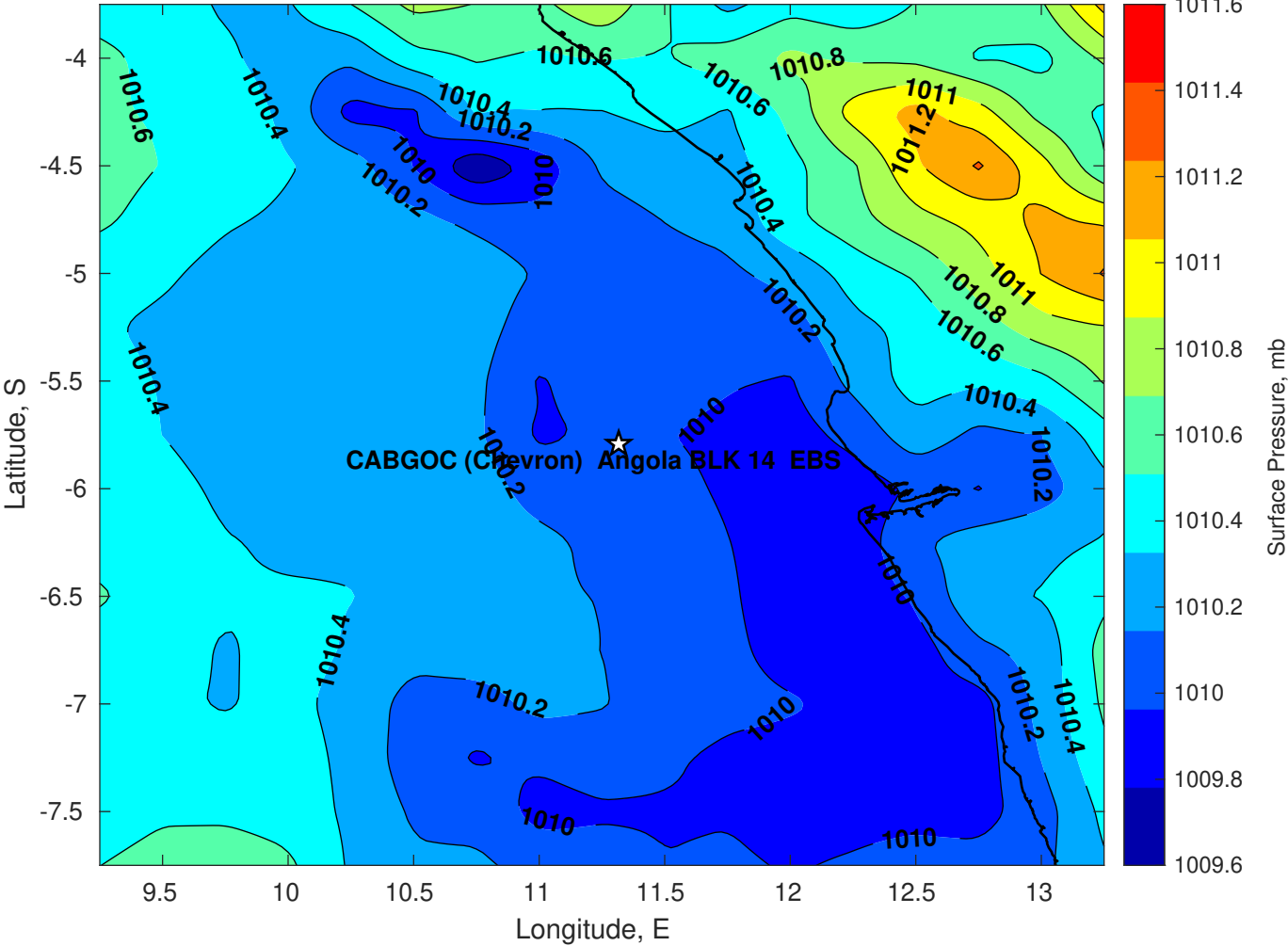
Surface Pressure (mb) for CABGOC (Chevron) Angola BLK 14 EBS at 26-Mar-2025 00:00:00
