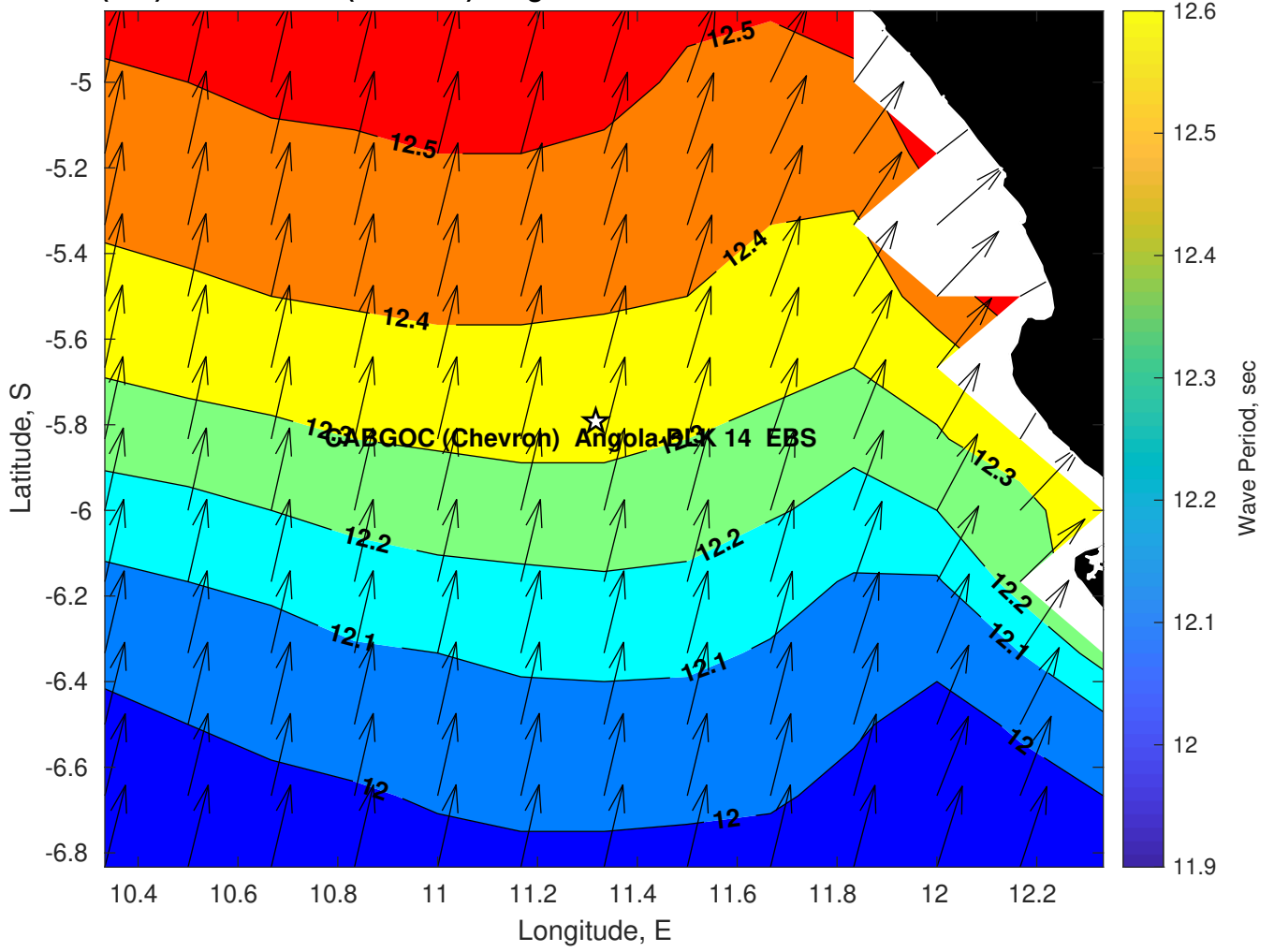
Wave Period (sec) for CABGOC (Chevron) Angola BLK 14 EBS at 26-Mar-2025 09:00:00
