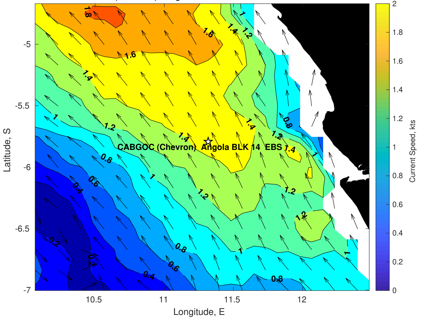
Surface Currents for CABGOC (Chevron) Angola BLK 14 EBS at 25-Mar-2025 00:00:00
