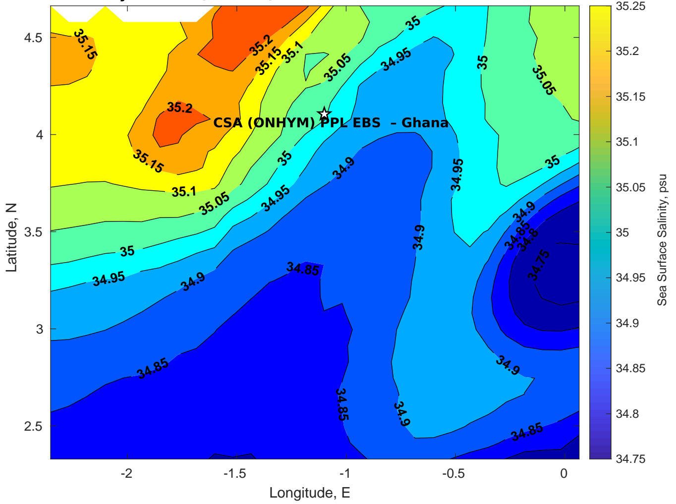
Surface Salinity for CSA (ONHYM) PPL EBS - Ghana at 25-Mar-2025 00:00:00
