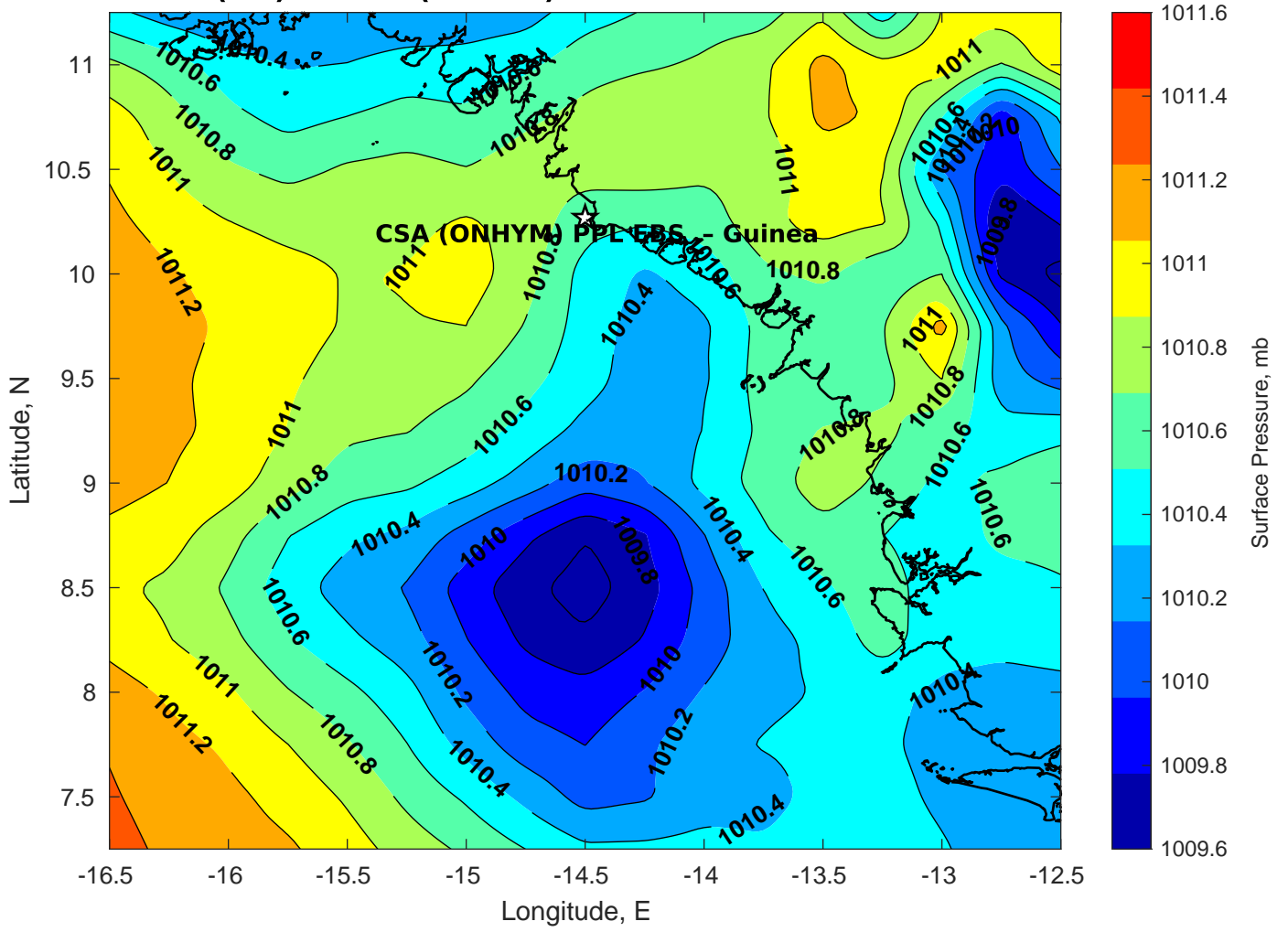
Surface Pressure (mb) for CSA (ONHYM) PPL EBS - Guinea at 27-Mar-2025 00:00:00
