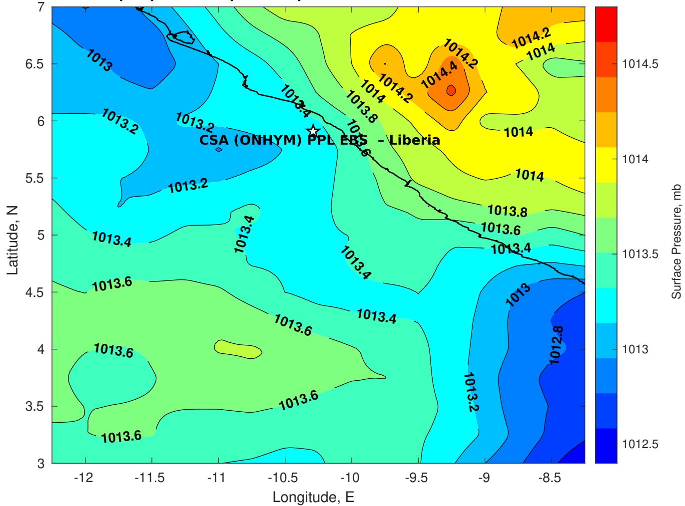
Surface Pressure (mb) for CSA (ONHYM) PPL EBS - Liberia at 26-Mar-2025 00:00:00
