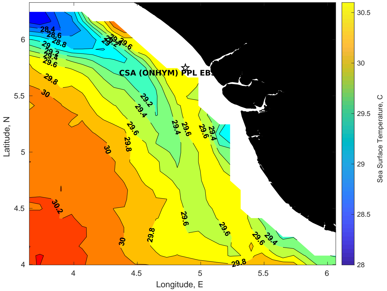
SST for CSA (ONHYM) PPL EBS - Nigeria at 25-Mar-2025 00:00:00
