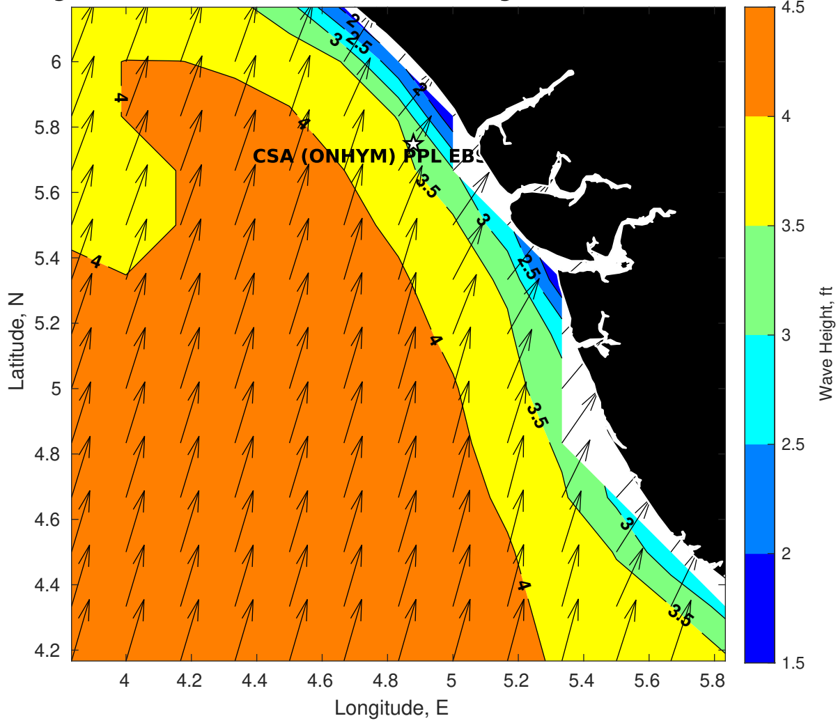
Wave Height (ft) for CSA (ONHYM) PPL EBS - Nigeria at 26-Mar-2025 09:00:00
