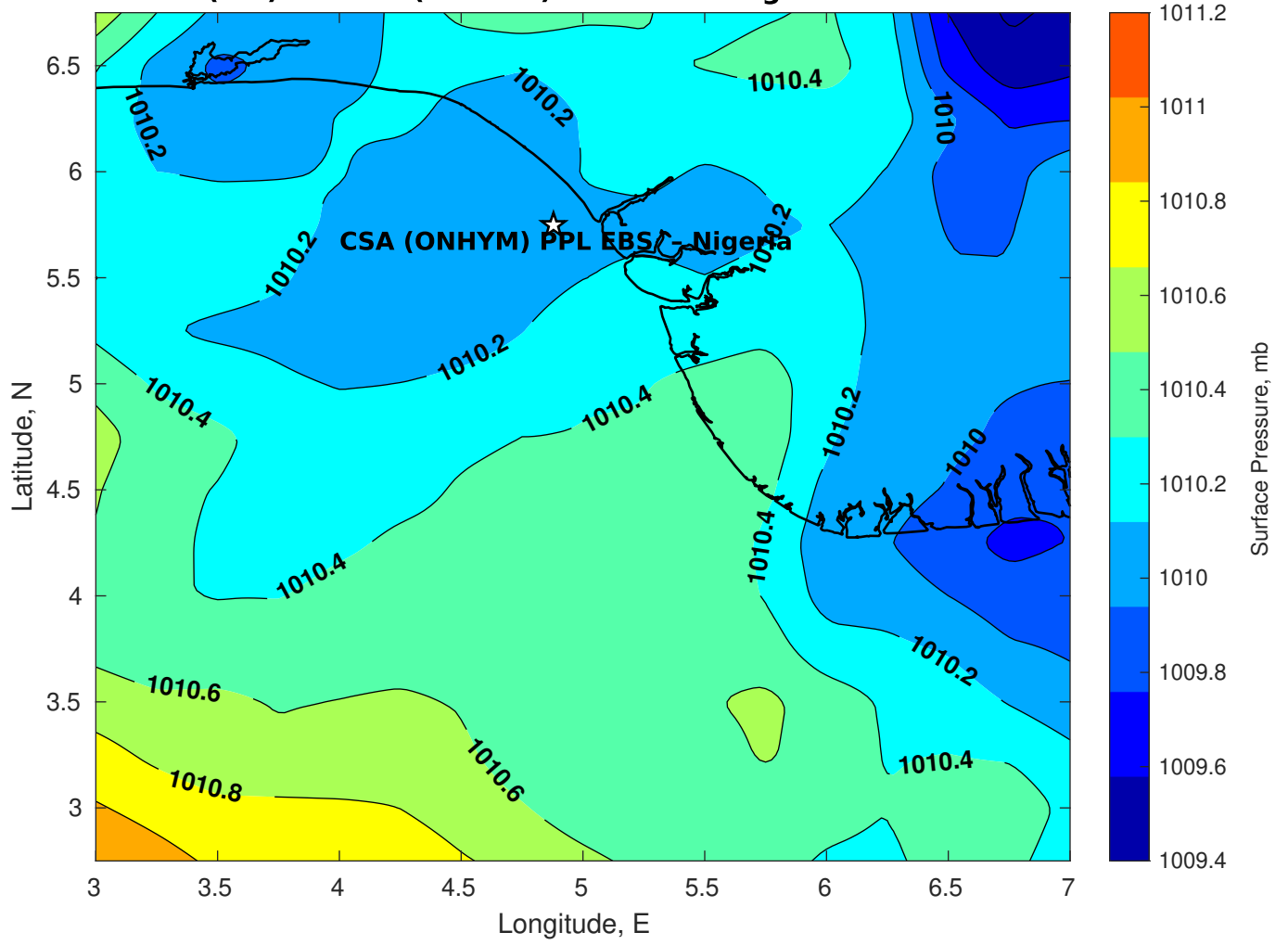
Surface Pressure (mb) for CSA (ONHYM) PPL EBS - Nigeria at 26-Mar-2025 00:00:00
